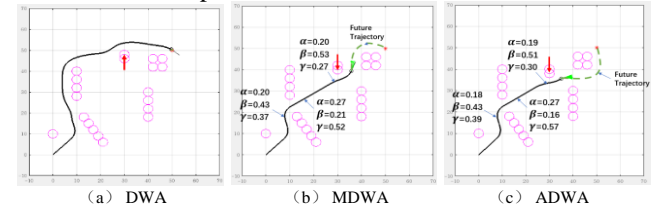
FIGURE 14. Simulation path in fusion obstacle environment
