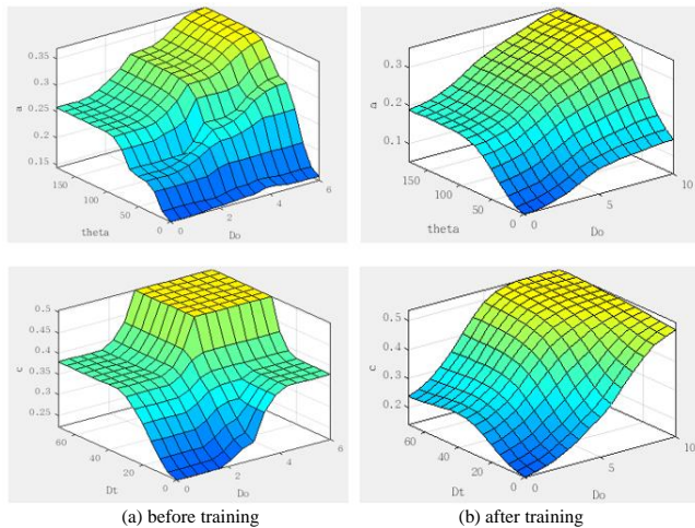
FIGURE 10. Comparison of fuzzy regular surfaces
