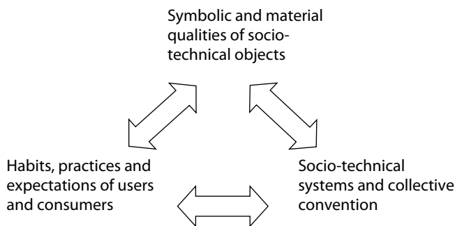
Figure 3.2. Three dimensions of co-evolutions (Shove, 2003a, p. 48).
