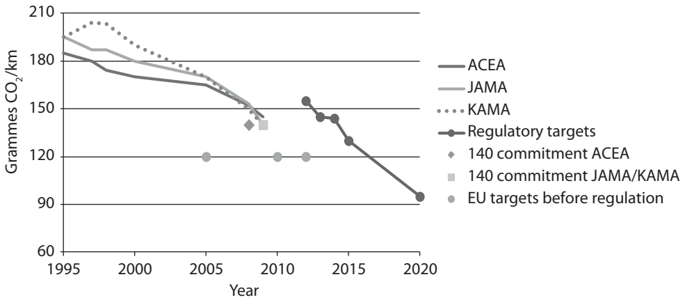
Figure 2.6. Progress over time in the CO 2 commitment of three car manufacturer associations in Europe, including historical and existing voluntary and regulatory targets (adapted from T&E, 2010).
