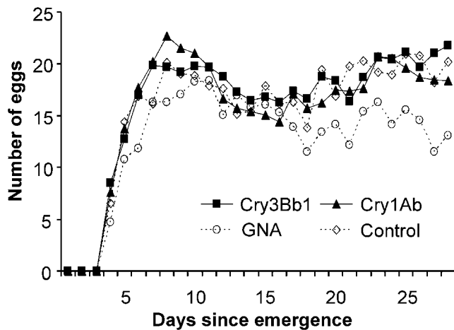
Figure 2. Mean daily fecundity of Chrysoperla carnea fed artificial diet containing insecticidal proteins. Per g dry weight, 150 \mu\text{g} Cry3Bb1, 120 \mu\text{g} Cry1Ab or 9 mg GNA (positive control) were incorporated. Pure diet served as a negative control. N=33-35 . doi:10.1371/journal.pone.0002909.g002
