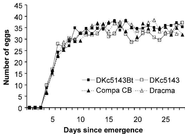
Figure 1. Mean daily fecundity of Chrysoperla carnea fed pollen from either of two Bt maize varieties or their respective non-transformed near isolines. Insects were provided 1 M sucrose solution together with pollen from: (a) DKc5143Bt expressing Cry3Bb1 (MON 88017), (b) the corresponding control DKc5143, (c) Compa CB expressing Cry1Ab (Event Bt176), and (d) the corresponding control Dracma. N = 30–34.
