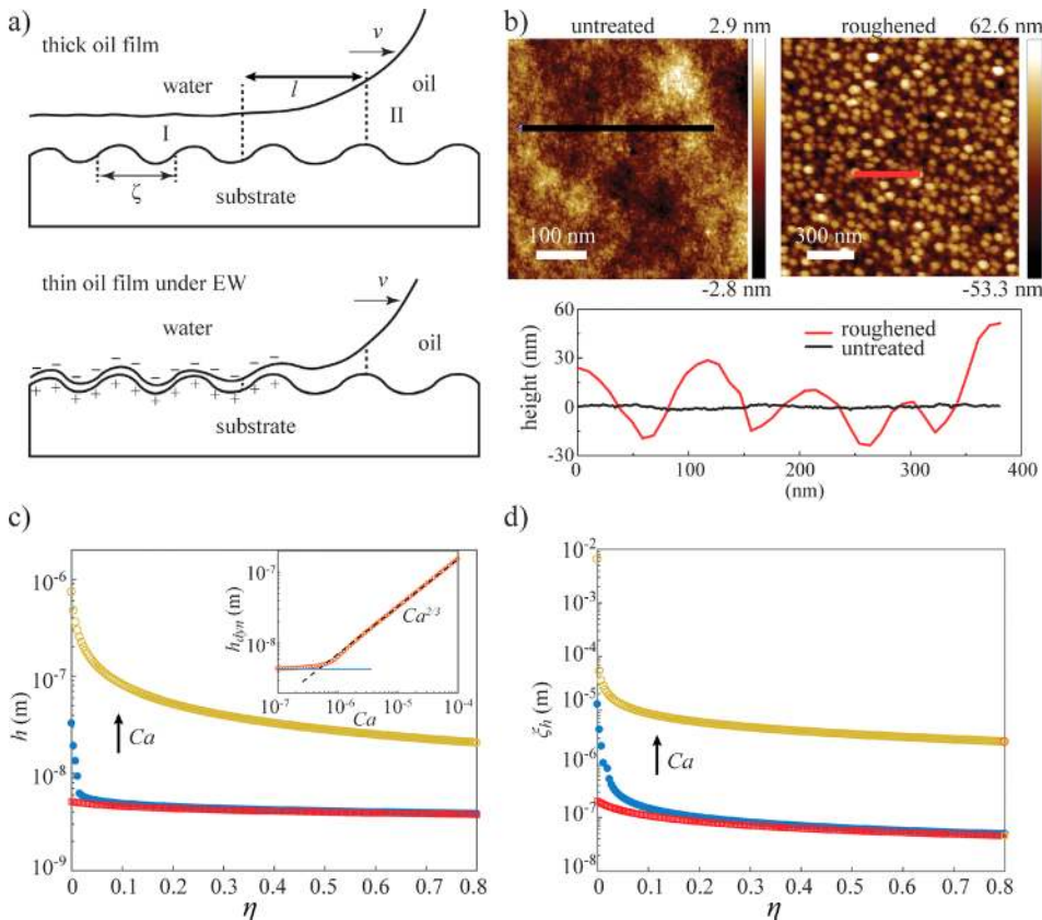
FIG. 3. Analysis of the mechanism. (a) Sketch of the oil film entrained between the water droplet and substrate, which follows the surface roughness profile. (b) AFM image of the untreated and roughened substrate. (c) h_{dyn} at Ca = 2 \times 10^{-5} (yellow open circles) and Ca = 2 \times 10^{-7} (blue solid circles), and h_{sta} (red open squares) for \eta = 0 \dots 0.8 . Inset: h_{dyn} for Ca = 10^{-7} \dots 10^{-5} at \eta = 0.2 . (d) \xi_{h-dyn} at Ca = 2 \times 10^{-5} (yellow open circles) and Ca = 2 \times 10^{-7} (blue solid circles), and \xi_{h-sta} (red open squares) for \eta = 0 \dots 0.8 .
