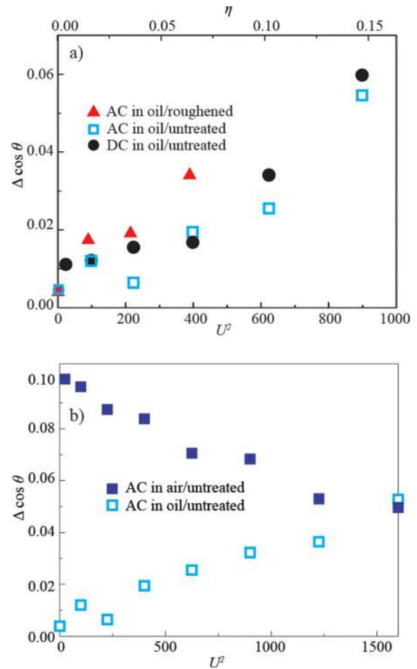
FIG. 2. \Delta \cos\theta vs. U^2 for the in-oil EW configuration (a) and comparison between \Delta \cos\theta vs. U^2 for ambient air vs. ambient oil (b).
