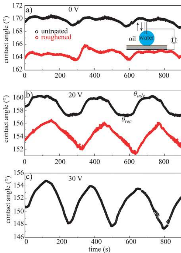
FIG. 1. Advancing and receding contact angles for (a) 0 V ( \eta=0 ), (b) 20 V ( \eta=0.065 ), and (c) 30 V ( \eta=0.147 ) under EW for the untreated substrate (black) and the roughened substrate (red). Note that higher than 20 V is not tested on the roughened substrate due to its comprised dielectric strength. The inset in (a): simplified sketch of the set-up (not to scale).
