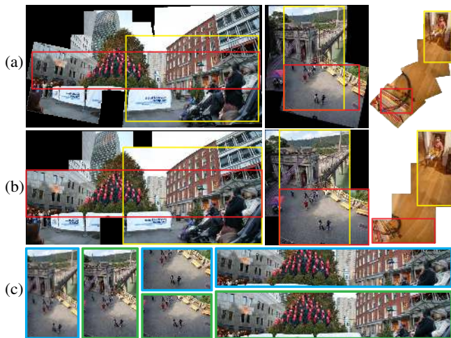
Figure 12. Results of challenging cases. (a) Initial stitching results with irregular boundaries, (b) results of our piecewise rectangling stitching, (c) cropped images based on the stitched panoramas of [4] (cyan border) and our results (green border).
