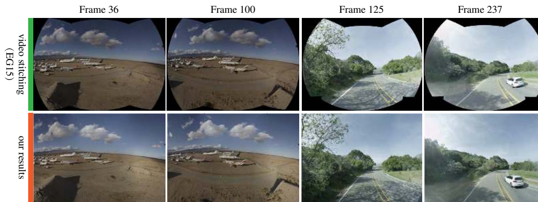
Figure 14. Application to rectangling video panoramas. We give two examples, and for each example show stitched panoramas of 2 different frames obtained by [17] and our method respectively.
