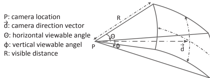
Fig. 1: Illustration of the 3D FOVScene model.
