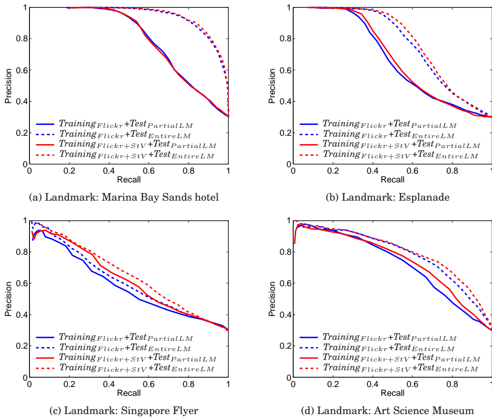
Fig. 6: Evaluations with two training sets (Flickr only or Flickr with Google StreetView images, Flickr+StV ) and two test sets (partial or entire view of landmarks) for the content-based ScSPM method.
