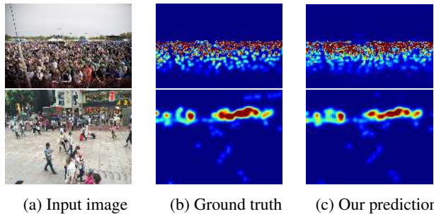
(a) Input image (b) Ground truth (c) Our prediction Figure 4: Crowd density estimation on ShanghaiTech. First row: Image from Part A. Second row: Image from Part B. Our model adjusts to rapid scale changes and delivers density maps that are close to the ground truth.
