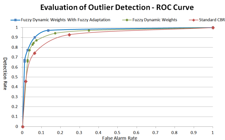
Fig. 10 ROC Space of Three Different Approaches for Anomaly Detection
