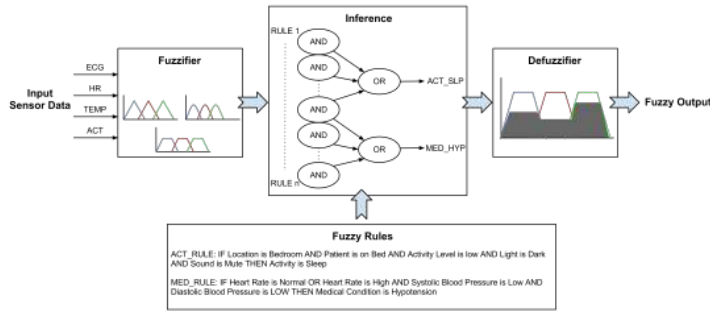
Fig. 1 A Fuzzy Logic System
