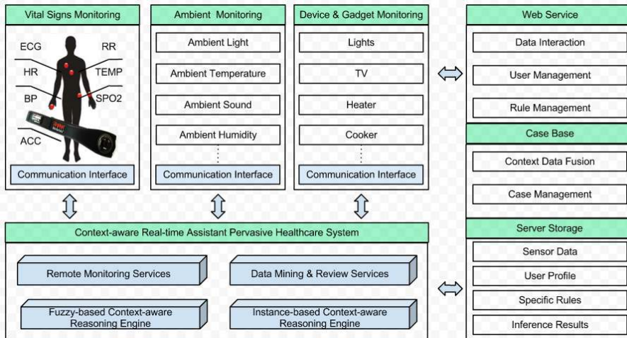
Fig. 4 Architecture of CARA System
