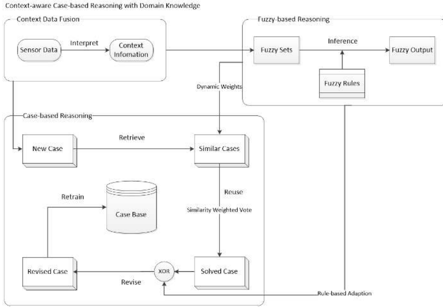
Fig. 7 The Structure of Context-aware Hybrid Reasoning Framework
