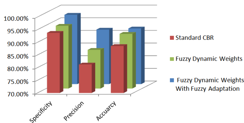
Fig. 11 Best Performance of Three Different Approaches
