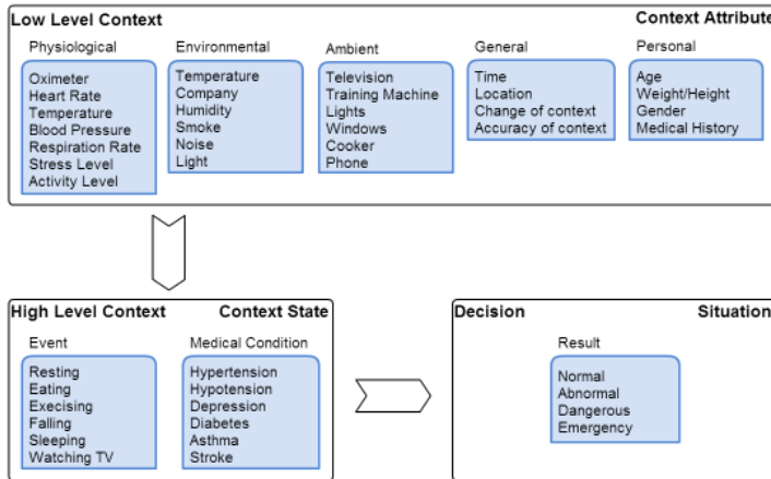
Fig. 6 Fuzzy Context Model
