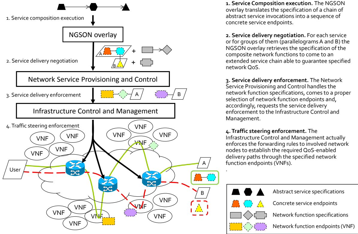
Fig. 4: NGSON service composition workflow extended with adaptive service delivery.
