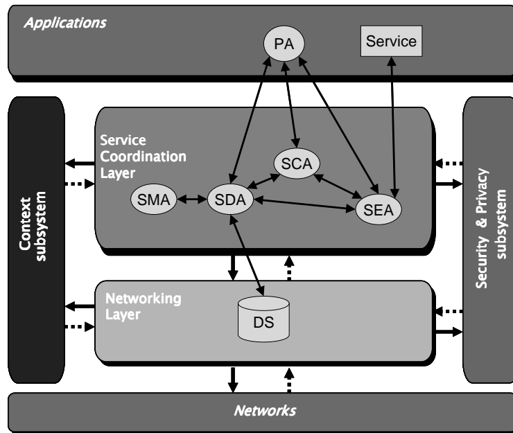
Figure 2: Layered model of the architecture (PA: Personal Agent, SMA: Service Matchmaking Agent, SDA: Service Discovery Agent, SCA: Service Composition Agent, SEA: Service Execution Agent, DS: Directory Service)
