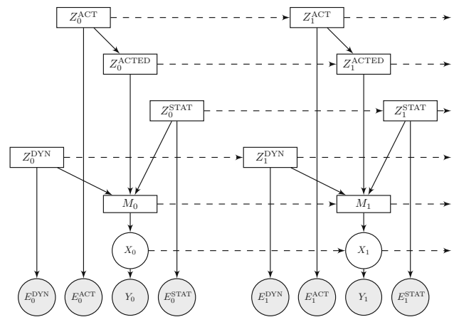
Fig. 5 DBN with context cues for VRU path prediction, unrolled for two time slices. Discrete/continuous/observed nodes are rectangular/circular/shaded. The binary context nodes represent interaction with the dynamic environment Z_t^{\text{DYN}} , relation to the static environment Z_t^{\text{STAT}} , and object behavior (i.e. how VRU acts, Z_t^{\text{ACT}} , or has acted, Z_t^{\text{ACTED}} )
