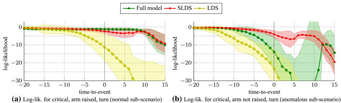
Fig. 14 Best viewed in color. Cyclist scenario: Prediction likelihood when predicting 16 time steps (~ 1 s) ahead on critical sub-scenarios where the cyclist turns. a Normal sub-scenario where the arm was raised. b Anomalous sub-scenario where the cyclist did not raise an arm to express intent
