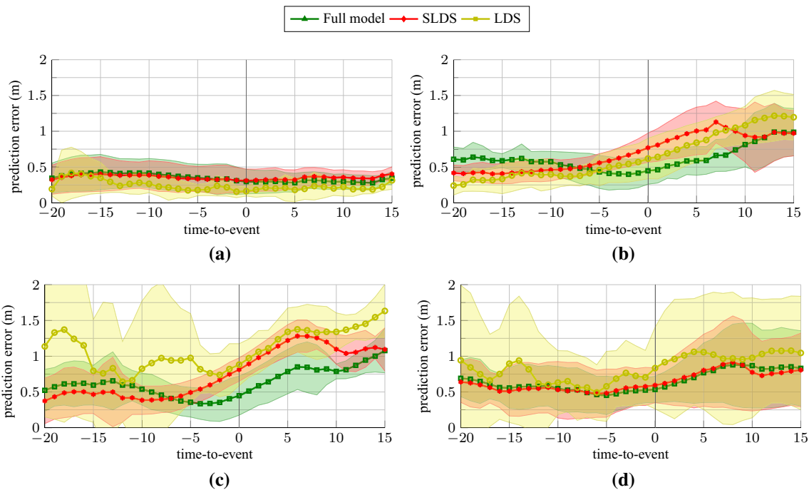
Fig. 13 Cyclist scenario. Prediction error on the normal sub-scenarios when predicting 16 time steps (~ 1 s) ahead. a Critical, arm not raised, straight. b Critical, arm raised, turn. c Non-critical, arm raised, turn. d Non-critical, arm not raised, straight/turn
