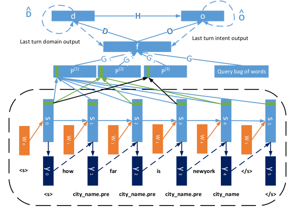
Fig. 1. RNN based contextual SLU.
