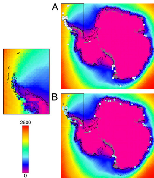
Fig. 2. Distribution of cumulative annual degree days for 2007–2008 in the Antarctic. These were calculated by using a -5^{\circ}\text{C} threshold and mean daily near-surface temperature data from the Modern Era Retrospective-analysis for Research and Applications Reanalysis office (provided by the NASA Global Modeling and Assimilation) (50) on a 0.67^{\circ} longitude \times 0.5^{\circ} latitude grid, interpolated to a 50-km square grid. Inset shows degree day detail on the Antarctic Peninsula. Ice-free ground is shown in gray. Ice-free landing data for tourists (A) and scientists (B) are shown.
