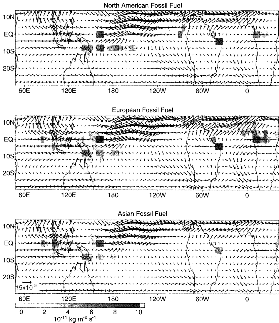
Figure 6. Simulated transport fluxes ( \text{kg m}^{-2} \text{s}^{-1} ) of tagged fuel CO from North America, Europe, and Asia at 10–13.5 km altitude. Shading indicates regions with large positive convective tendencies as diagnosed by increases in the 10–13.5 km column of CO ( \text{kg m}^{-2} \text{s}^{-1} ) due to convection.
