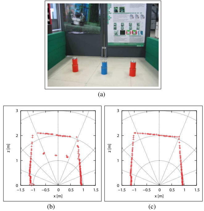
Fig. 4. Demonstration of the map types in an example scenario (a). The obstacle map (b) is generated by extracting minimum distances (projected into 2D) in the continuously acquired 3D data. Extracting maximum distances results in the structure map (c).
