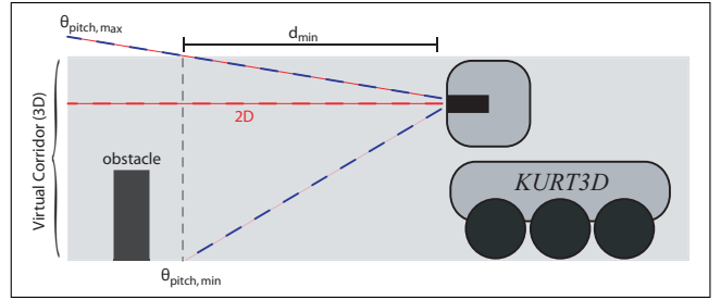
Fig. 2. Perception of the Virtual Corridor. Obstacles of different sizes can be perceived in contrast to standard 2D perception. \theta_{pitch, min} and \theta_{pitch, max} are chosen in a way to represent the minimal Area Of Interest (AOI) .
