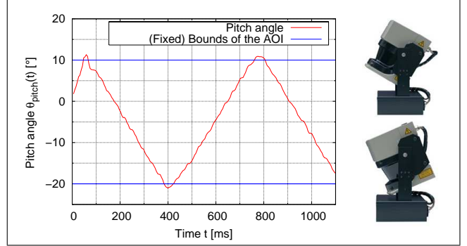
Fig. 3. Sequence of pitch angles \theta_{pitch} to continuously sense the Area Of Interest (AOI) . Lower and upper bound of the AOI as well as the scanner's pitch rate are exemplarily fixed.
