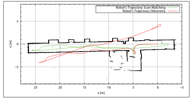
Fig. 6. 2D Map of a 30 m long corridor. The data for matching was extracted from the continuous 3D data flow.
