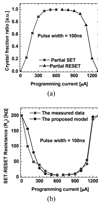
Fig. 4. (a) Crystal fraction ratio vs. programming current plot, (b) Comparison between the measured [1] and simulated resistance in the full SET, full RESET, partial SET, and partial RESET states.
