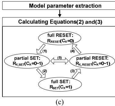
Fig. 1. (a) Current-voltage characteristic of PCRAM with 3 operation regions of SET-RESET, Negative Differential Resistance (NDR), and ON, (b) Comparison between the measured data [1] and the previous PCRAM model Eq. (1) in [10]. The partial state ( R_X=20 \text{ k}\Omega ) that is close to the full SET state ( R_X=7 \text{ k}\Omega ) shows a very large discrepancy between the measurement and the model Eq. (1) in [10], (c) Flow chart of the proposed PCRAM Verilog-A model where (1) means that the full RESET state changes to the partial SET and (2) means that the partial SET changes to the full SET. Similarly, the full SET changes to the partial RESET via (3) and the partial RESET changes to the full RESET via (4). (5) means the partial SET changes to the partial RESET and vice versa.
