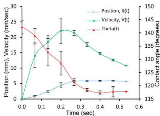
Figure 6. Droplet transport characterization on dry surface: contact angle, position, and velocity. The droplet is deposited on the outer region and is self-propulsed toward the center.
