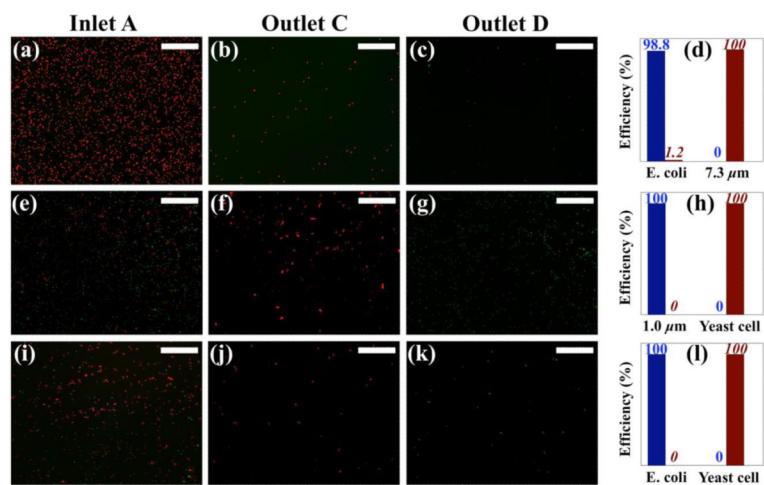
Figure 5. Experimental composite micrographs of size distribution analysis, including micrographs of particles/cells mixture collected before sorting at Inlet A and after separation at Outlets C and D, and remaining and separation efficiencies. (a) – (d) were for Escherichia coli and 7.3 \mu\text{m} particles mixture; (e) – (h) were for Saccharomyces cerevisiae and 1.0 \mu\text{m} particles mixture; (i) – (l) were for Escherichia coli and Saccharomyces cerevisiae mixture. Blue bar with normal number on top shows remaining efficiency, while red bar with italic number on top shows separation efficiency. Scale bars represent 200 \mu\text{m} .
