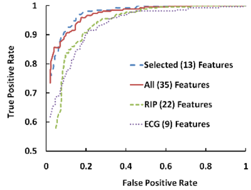
Figure 8: ROC curves for the best classifiers when using all 35 features, 13 selected features, only the 9 ECG features, and only the 22 RIP features. The curves show that performance of classifiers using all features and a subset of features are comparable with Area Under ROC Curve (AUC) being 0.964 and 0.967 respectively (with 1 being the best possible value). Also, RIP features have similar discriminatory power as ECG features (AUC for ROC curves being 0.924 and 0.926 respectively).
