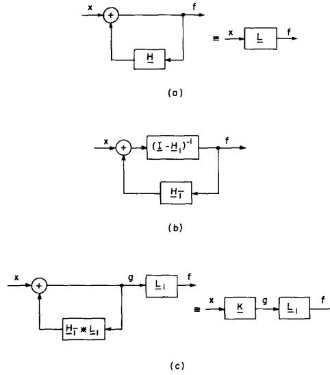
Fig. 22. Block-diagram manipulation: (a) feedback system; (b) first equivalent system; (c) second equivalent system.
