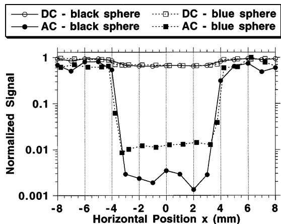
Fig. 3. One-dimensional images of a black and a blue glass sphere obtained with the dc unmodulated laser-light signals and the ac ultrasound-modulated laser-light signals.
