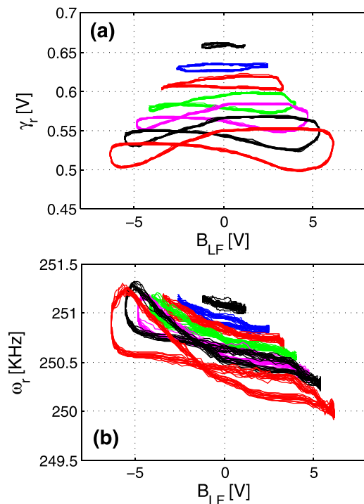
FIG. 3. Resonance amplitude \gamma_r and resonance frequency \omega_r as a function of the strain amplitude induced by the pump.
