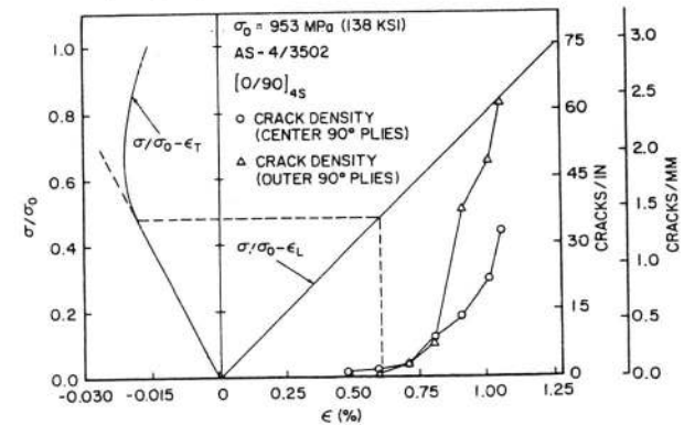
Fig. 6. The Kistner et al. data showing stress-strain behavior and associated transverse crack density of a graphite-epoxy (0,90)_4S laminate.
