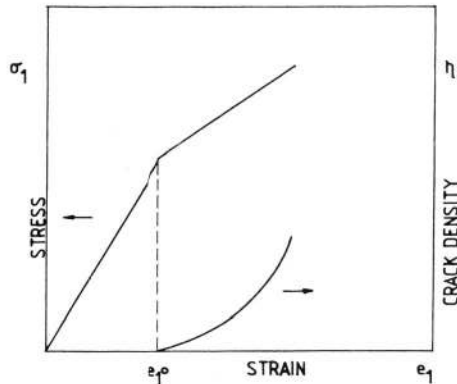
Fig. 3. A bilinear stress-strain behavior with associated development of transverse crack density.
