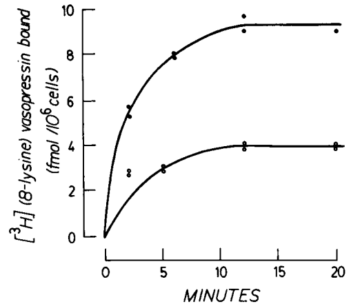
FIGURE 4 Time-course of [ ^3\text{H} ]LVP binding to a broken MS-cell preparation. Six culture dishes ( 24 \times 10^6 cells) of monolayer cells were washed with PBS and scrapped at 4^\circ\text{C} into 5 mM Tris-HCl, pH 7.4, containing 1 mM EDTA, and homogenized. The pooled homogenates were centrifuged at 10,000 g for 15 min and the pellet resuspended in homogenizing buffer. Sample aliquots were incubated for various periods of time with either 5 nM ( \bullet ) or 1.6 nM ( \circ ) [ ^3\text{H} ]LVP in the absence or presence of 2 \mu\text{M} AVP. Specific binding, determined as described in Methods, is plotted vs. time. Data of duplicate assays are illustrated at each time point.
