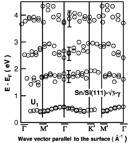
FIG. 9. Experimental band dispersion of the \gamma\sqrt{3} reconstruction. Electron energy is plotted against the wave vector parallel to the surface.
