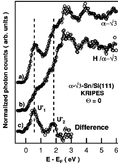
FIG. 5. (a) and (b) Kripes spectra of the \alpha phase respectively obtained before and after exposure of the sample to 1L of atomic hydrogen. (c) Difference curve (a),(b).
