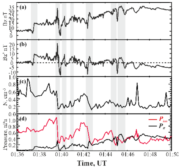
Figure 2. A zoom of the B_Z (a) and B_Z^* (b) fields, ion density (c), ion ( P_{\text{ion}} ) and magnetic ( P_B ) pressure (d) observed by C4 during the dipolarization growth. The intervals of strong B_Z pulses are shaded grey.
