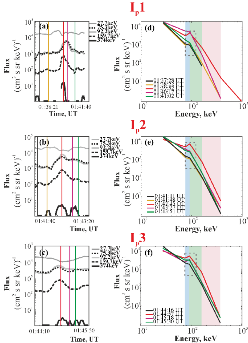
Figure 6. The observations of proton fluxes and spectra by the C4 spacecraft. The format is similar to the format of Fig. 4 except for wave data.
