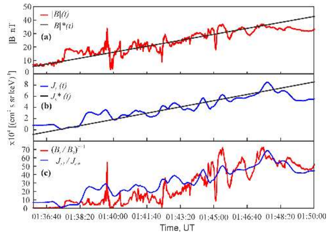
Figure 8. Panels (a–c) show the time profiles of the absolute value of the magnetic field |B|(t) and electron flux J_e(t) at 50.5 keV displayed along with the linear approximations |B|^*(t) and J_e^*(t) , respectively (for explanation, see Sect. 6). In (c) the time profiles of J_{ei}(t)/J_{e1} and (B_i(t)/B_1)^{\gamma+1} are shown (for explanation, see Sect. 6.2).
