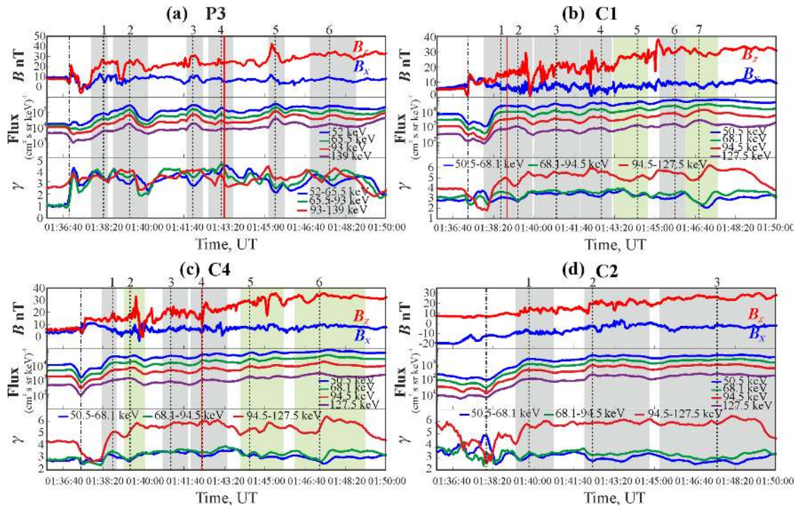
Figure 3. The dynamics of suprathermal electron fluxes and spectral index \gamma observed by P3, C1, C4 and C2 satellites. In each plot the following data from a given spacecraft are shown from top to bottom: the time profiles of B_X and B_Z magnetic field components, the time profiles of electron fluxes in several energy ranges and the spectral index \gamma calculated for three energy ranges indicated in the corresponding panel. The time moment of dipolarization onset at each spacecraft is shown by the vertical dashed and dotted line. The intervals of dispersed injections are shaded light green and the intervals of dispersionless injections are shaded grey. The moments of peak electron flux observations in each injection are indicated by vertical dashed lines. The moments of \gamma variations which cannot be explained by the time-of-flight energy dispersion are indicated by red solid vertical lines.
