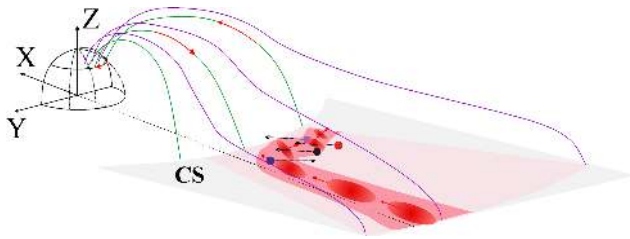
Figure 7. A diagram of the observed magnetic structure of the flux pile up region in the near-Earth PS. An area shaded light pink represents the perturbed CS. The localized area shaded dark pink displays a channel in which the multiple BBFs with the embedded DFs (shown by red ovals) propagate. The direction of DFs’ motion is shown by red arrows. P3 probe and Cluster spacecraft are shown by colored dots and their trajectories during the event are shown by black dotted arrows. Near the P3 and Cluster locations the multiple BBFs are braked and diverted. The system of field-aligned currents and westward electrojet is shown by red arrows.
