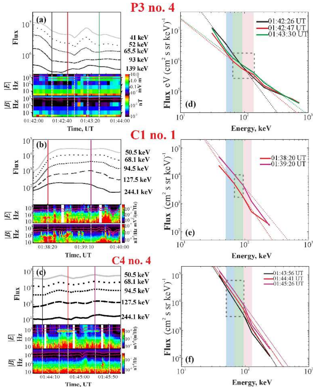
Figure 4. The observations of electron fluxes, spectra and wave activity obtained by P3, C1 and C4 spacecraft. Panels (a–c) show the time profiles of electron fluxes and frequency spectrograms of the power density of electric and magnetic field fluctuations observed by a given spacecraft within short time intervals around the moments marked by red vertical lines in Fig. 3. The solid magenta lines in frequency spectrograms display the time profiles of f_{ce} and 2f_{ce} . Panels (d–f) show the electron spectra observed by a given spacecraft at the time moments indicated in the left plots by vertical lines of the corresponding color. The colored bars shows three energy ranges for which the spectral index \gamma was calculated. The dashed bars indicate the transient features in energy spectra.
