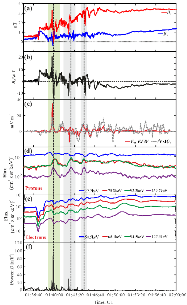
Figure 5. From top to bottom the following data observed by C4 spacecraft are shown: the time profiles of B_X and B_Z components (a); the time profile of B_Z^* (b; see explanations in the text), the dawn–dusk electric field (c), proton fluxes in several energy channels (d), fluxes of suprathermal electrons for the reference (e) and the time profile of the power of magnetic field fluctuations at proton gyrofrequency (f). The interval of the dispersed proton injection is shaded light yellow and the intervals of dispersionless injections are shaded grey. The moments of peak proton flux in each injection are shown by vertical dashed lines.
