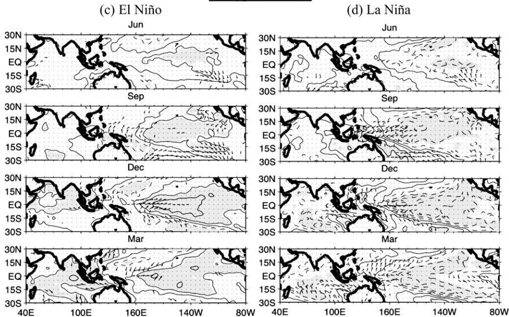
FIG. 12. Composite of SST and surface winds anomalies for (a) EP-El Niño, (b) EP-La Niña, (c) CP-El Niño, and (d) CP-La Niña events referenced to the calendar month. Wind vectors are shown and SST are shaded when they pass the 95% Student's t significance test.
