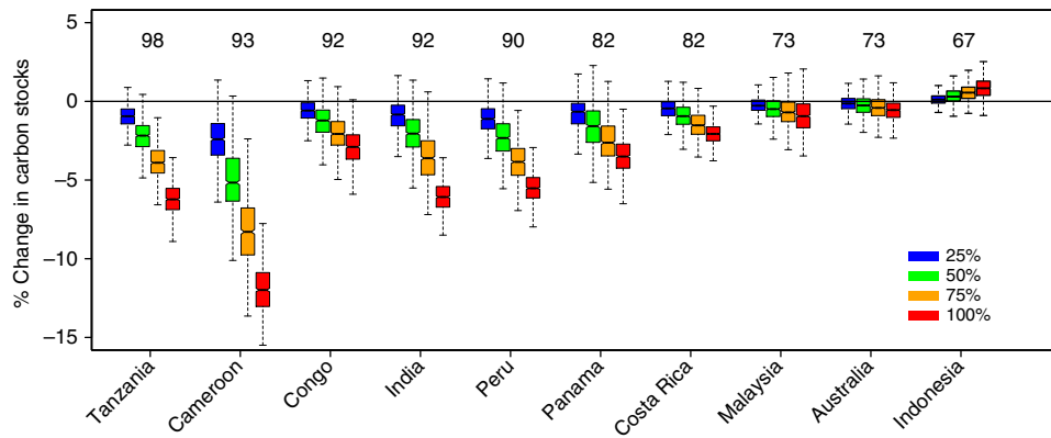
Figure 1 | Effects of simulated removal of large-seeded animal-dispersed species on aboveground carbon storage. Box-and-whisker plots depicting changes relative to original carbon stocks for 1,000 simulation runs following removal of 25, 50, 75 and 100% of individuals belonging to large-seeded animal-dispersed tree species. Numbers above boxes represent the relative abundances (%) of animal-dispersed species at each site.
