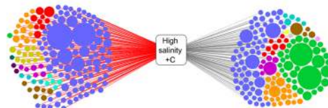
Figure 4. SVs responding to soil salinity. Circles represent SVs colored according to their phylum-level classification and sized by their average relative abundance. Lines connect SVs to treatments in which their abundance changed significantly compared to the control with the corresponding carbon treatment. Black lines indicate significant increase, red lines significant decrease.
