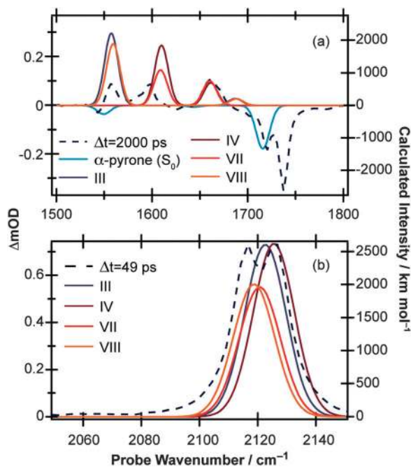
Fig. 7 Simulated IR spectra for the four ring-open E -isomers of \alpha -pyrone calculated at the B3LYP/6-311++G(d,p) level of theory with implicit solvation accounted for using the PCM method. Panels (a) and (b) cover the 1500–1800 \text{cm}^{-1} and 2050–2150 \text{cm}^{-1} regions, respectively. The solid lines are the computed spectra (represented by Gaussian functions with 10 \text{cm}^{-1} FWHM), and the dashed lines are the experimental data recorded at time delays of 2000 ps and 49 ps in (a) and (b), respectively.
