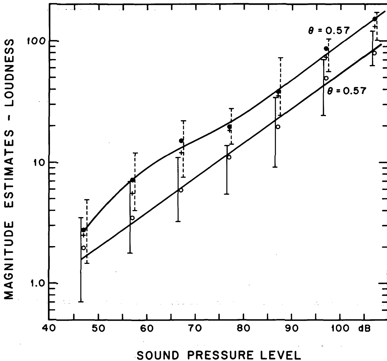
Figure 1. Loudness-estimation function produced by broadband-flat noise (upper solid line) compared to the one produced by a 1000-Hz tone (lower solid line). Filled circles and crosses indicate group geometric means of 22 judgments obtained for noise one week apart by the same group of eleven listeners. Unfilled circles indicate group geometric means of 22 judgments at 1000 Hz by the eleven listeners who also judged the noise. Solid and intermittent vertical bars show the interquartile ranges obtained for tone and noise respectively.
