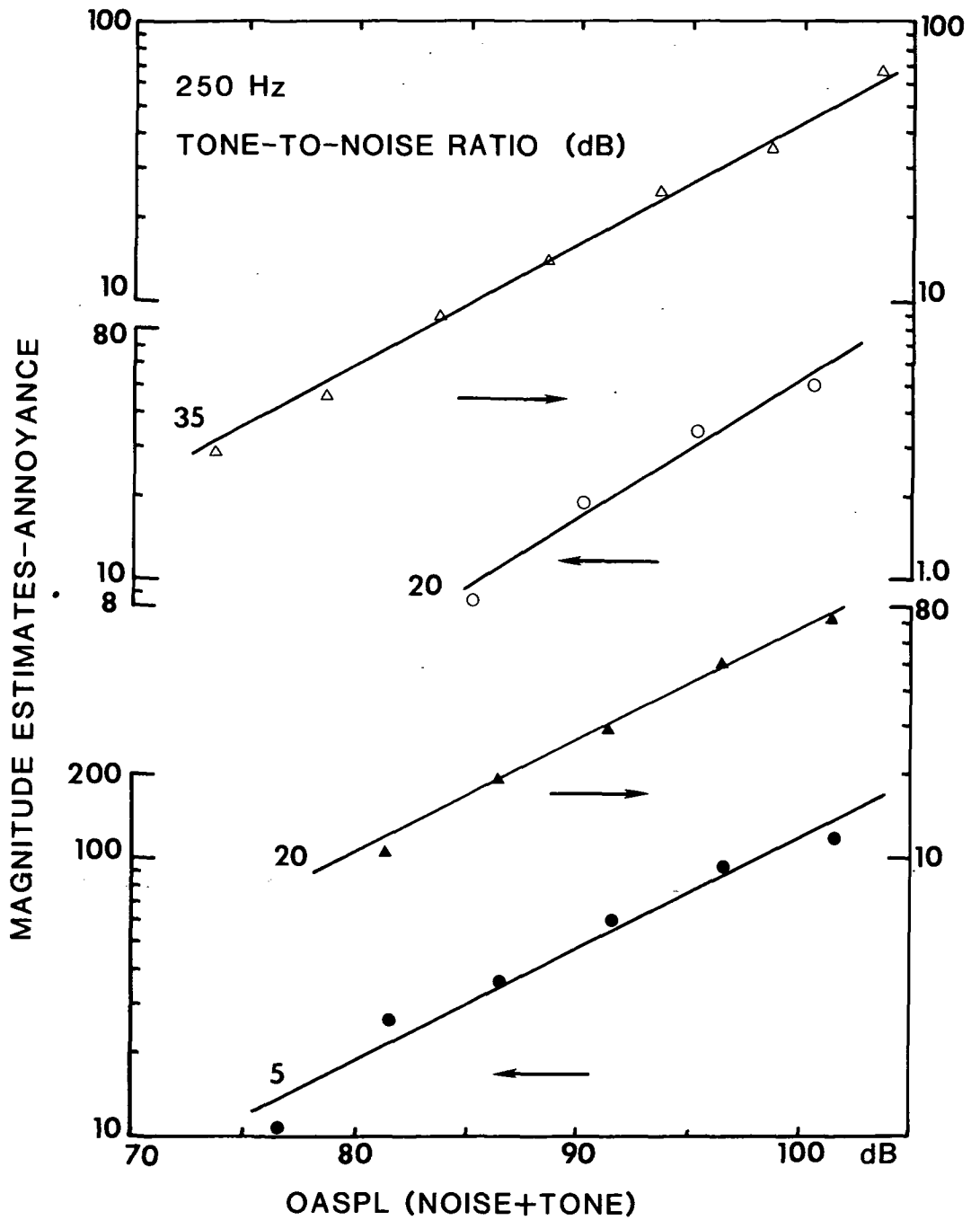
Figure B-4. Annoyance growth rate at 250 Hz. Filled and unfilled symbols indicate results obtained with low- and high-pass noise, respectively. With low-pass noise, group means at tone-to-noise ratios of +5 and +20 dB (filled circles and triangles) are shown. With high-pass noise, group means at tone-to-noise ratios of +20 and +35 dB (unfilled circles and triangles) are shown. All results are approximated by power functions of sound pressure.
