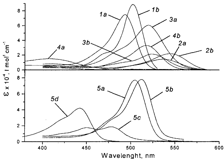
Fig. 2. Absorption spectra at p\alpha_{\text{H}^+}^* 6.9 of dianions (g, i) (1a-5a) mixture and calculated spectra of monoanions (f, h) (1b-5b) of substances (I) – 1a, 1b; (III) – 2a, 2b; (IV) – 3a, 3b; (V) – 4a, 4b; (II) – 5a, 5b; 5c – mixture of neutral forms (c,d), 5d – cation of substance (II). Spectra in 50% aqueous ethanol, as a rule at ionic strength 0.05 M (5c – at 5 M \text{H}_2\text{SO}_4 , 5d – at 18 M \text{H}_2\text{SO}_4 ).
