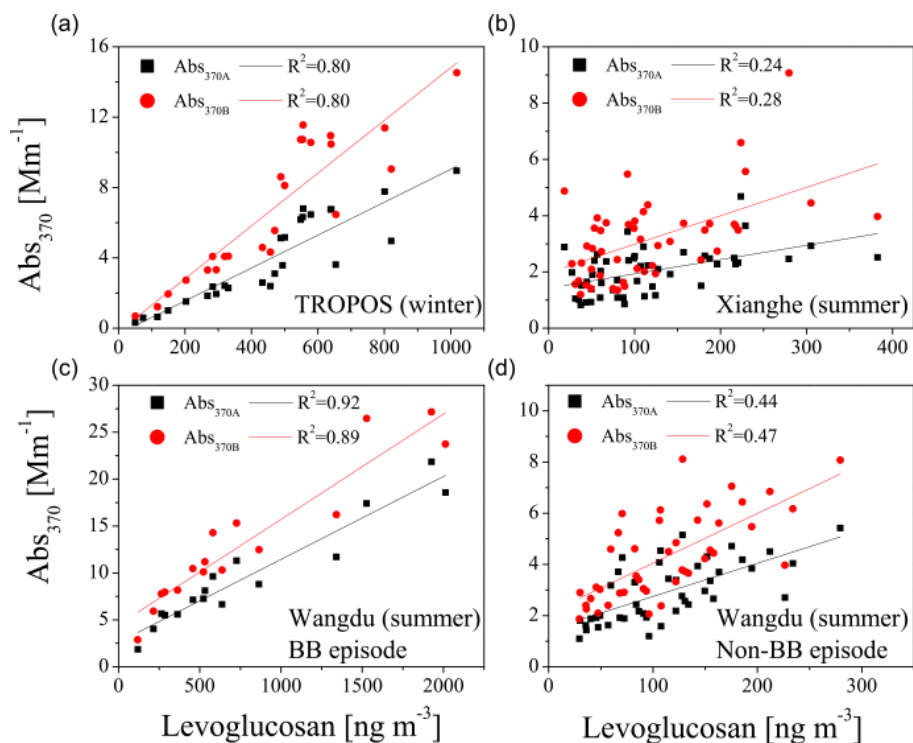
Figure 2. Scatter plot of the aqueous light absorption coefficient Abs_{370} with levoglucosan concentration for the campaigns (a) TROPOS (winter.), (b) Xianghe (summer), (c) Wangdu (summer, BB episode) and (d) Wangdu (summer, non-BB episode). Abs_{370} is given for acidic conditions (indicated by the subscript “A”, black squares) and for alkaline conditions (indicated by the subscript “B”, red dots). Note different axis scales.
