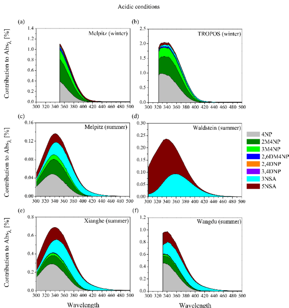
Figure 5. Relative contribution of NACs to Abs_{\lambda} over the spectral range of 300 to 500 nm for each measurement campaign (a–f) under acidic conditions. The data are presented as campaign averages. Due to instrumental issues, data for lower wavelengths are not always available.
