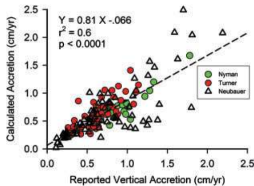
Figure 2. Mixing model-calculated accretion rates and reported 137 Cs-based vertical accretion rates. Calculations used published mass accretion rates ( \text{g m}^{-2} \text{yr}^{-1} ) of inorganic and organic matter as reported in Nyman et al. [1993, 2006], Turner et al. [2000], and Neubauer [2008].
