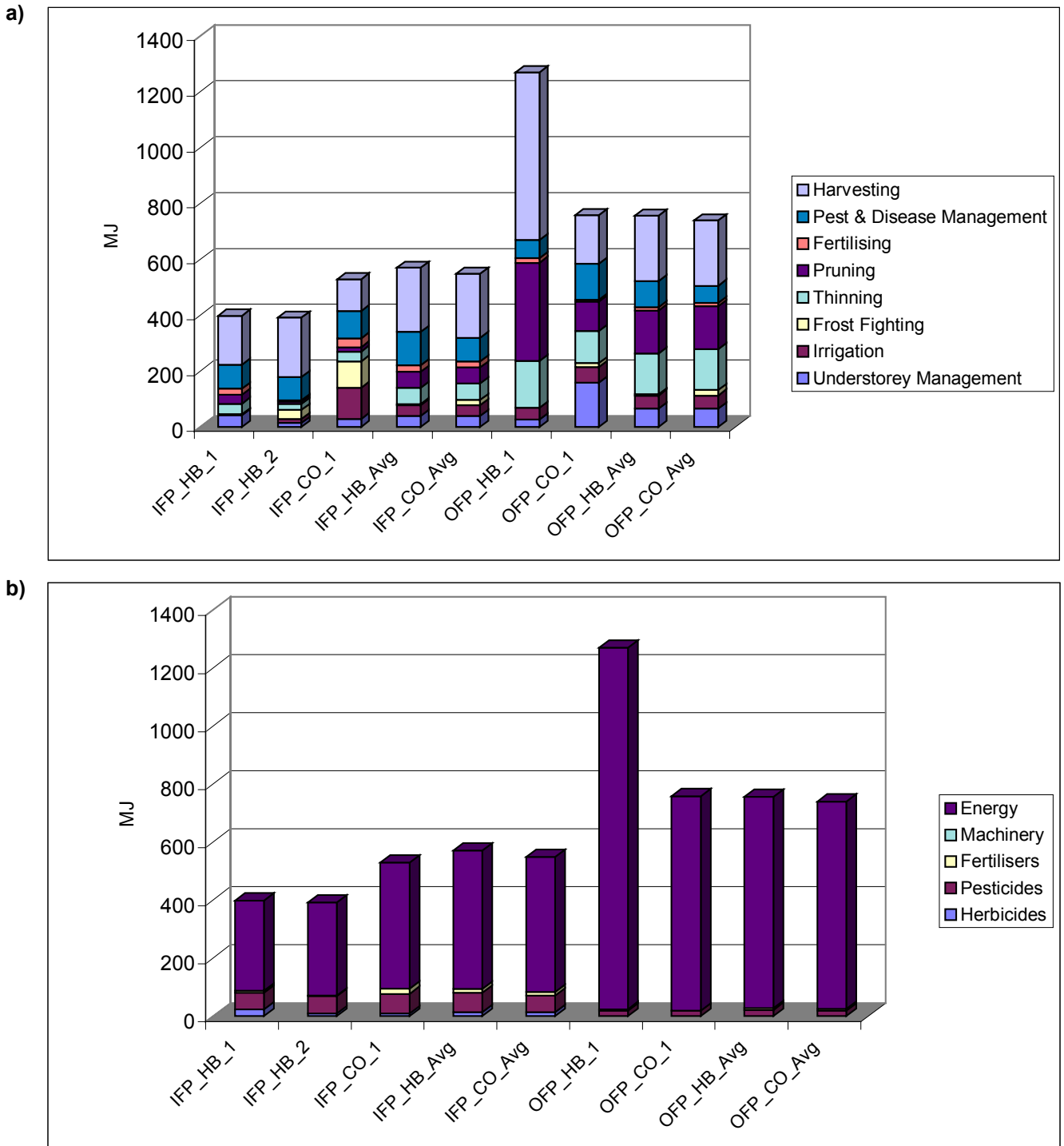
Figure III-9: a) Energy consumption in different field operations. b) Energy consumption by different input items. Results refer to 1 ton of apples of export or local quality.
