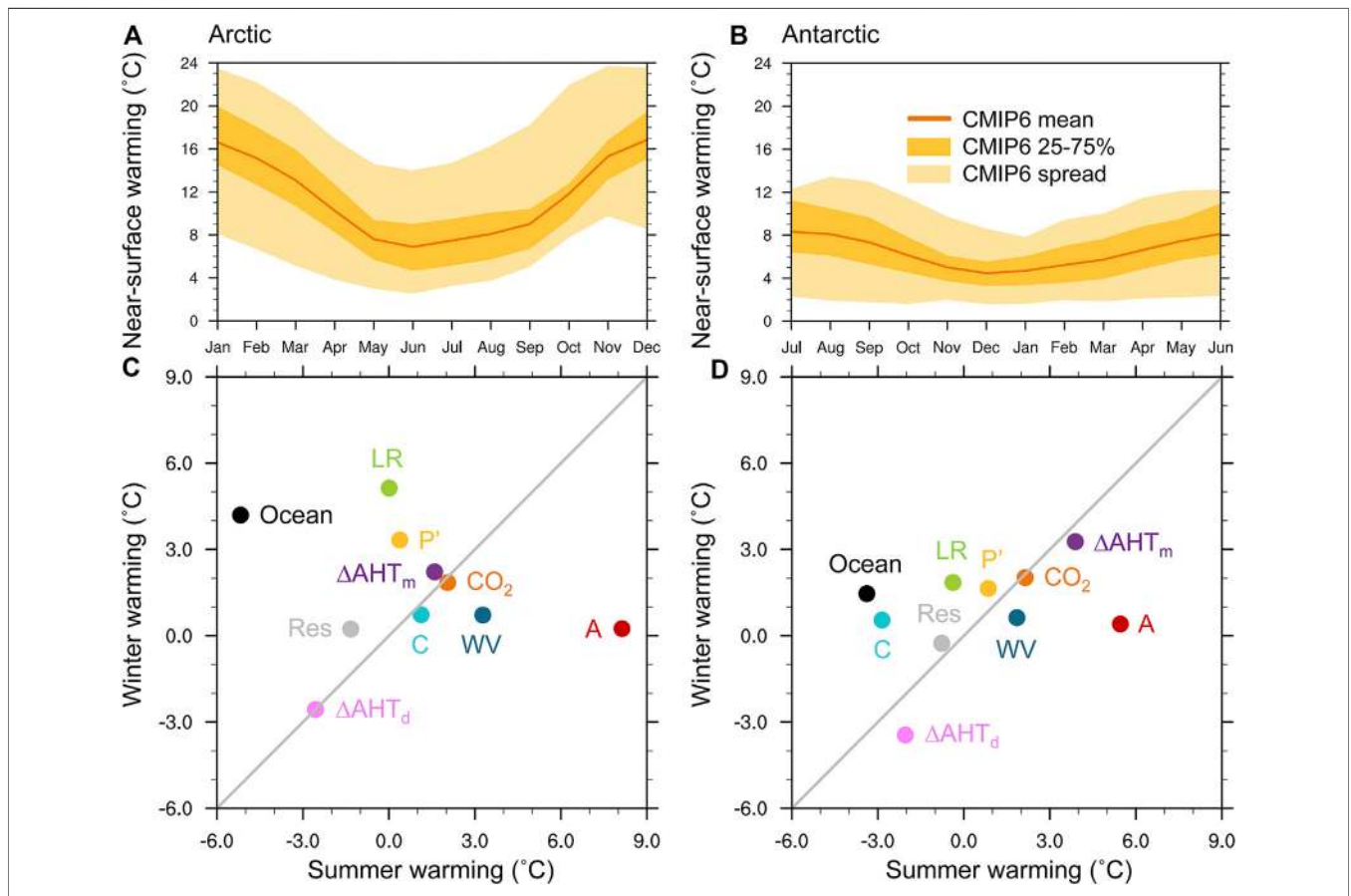
FIGURE 8 | Monthly near-surface warming (°C) centered around year-100 of abrupt CO_2 quadrupling for the CMIP6 multimodel mean (orange line), the 25th to 75th percentile (dark orange shading), and the full intermodel spread (light orange shading) in (A) the Arctic and (B) the Antarctic. (C, D) Contributions to winter and summer warming (°C) centered around year-100 of abrupt CO_2 quadrupling in CMIP6 for (C) the Arctic and (D) the Antarctic. Warming contributions are shown for the lapse-rate (LR), surface albedo (A), water-vapor (WV), and cloud (C) feedbacks, the variation in the Planck response from its global-mean value (P), effective radiative forcing ( CO_2 ), change in moist and dry AHT convergence ( \Delta AHT_m , \Delta AHT_d ) and ocean heat uptake (Ocean), and residual term (Res).
