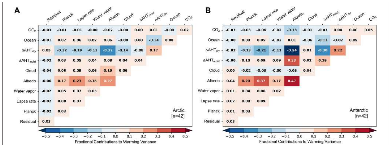
FIGURE 7 | Fractional contributions of each warming contribution term to intermodel variance in (A) Arctic and (B) Antarctic warming in CMIP6.
