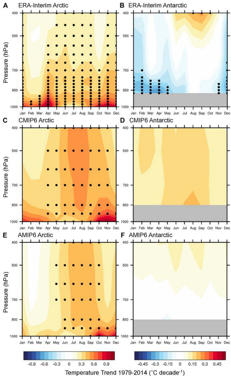
FIGURE 3 | Atmospheric temperature trends ( ^{\circ}\text{C decade}^{-1} ) for 1979–2014 for (A,C,E) the Arctic and (B,D,F) the Antarctic in the ERA-Interim reanalysis (A,B) , and historical CMIP6 (C,D) and AMIP6 (E,F) multimodel mean trends. Black dots in (A,B) show statistically significant trends at the 95% level based on a two-tailed Student’s t-test, and black dots in (C,D) and (E,F) show where 75% of models meet these criteria for significant trends. For the reanalysis and models, temperature data is first masked at pressures greater than the surface pressure, and trends are only shown where more than 50% of area-averaged grid points are non-missing.
