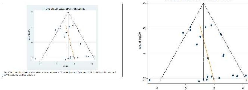
Figure 7.4: The original depiction of a funnel plot [left, reproduced under CC BY license from 10.1186/s13027-016-0058-9] and the manually extracted part that is subsequently ingested into the norma software (right).
