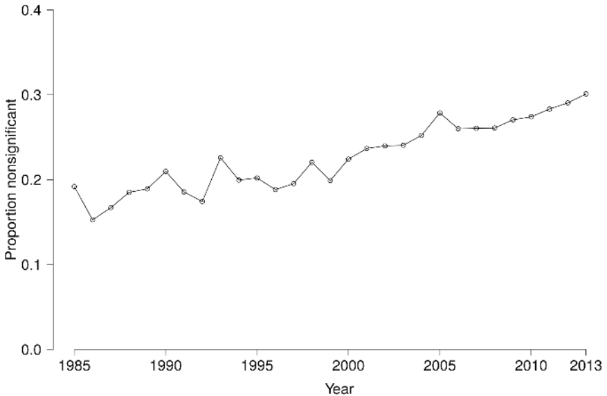
Figure 4.2: Observed proportion of nonsignificant test results per year.
