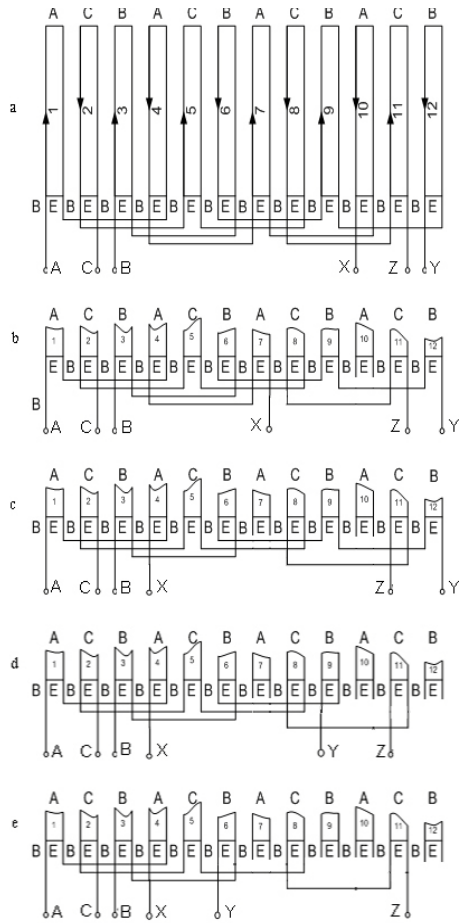
Fig. 2. Connection diagrams of CLIM coil windings
