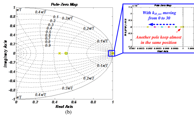
Fig. 13. pole-zero map for phase restoration. (a) PZ map with variable k_{pd\_sec} . (b) PZ map with variable k_{it\_sec} .
