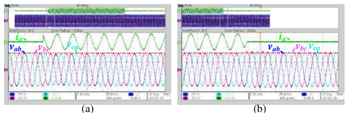
Fig. 26. UPS line to line voltage (phase a to b ) and phase a current (Voltage: 250V/Div, Current: 5A/Div). (a) Balanced load connected. (b) Balanced load disconnected.
