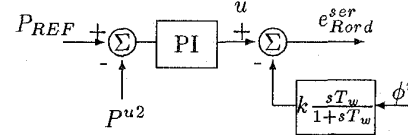
Figure 5: Real Power Controller
