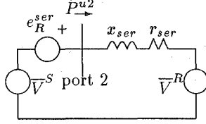
Figure 3: Simplified system
