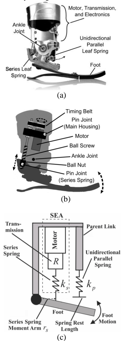
Fig. 1. Physical system with labeled components (a), diagram of the drive train (b), and mechanical model (c) of the powered ankle-foot prosthesis. The rotary elements in the photograph are shown as linear equivalents in the model schematic for clarity.
