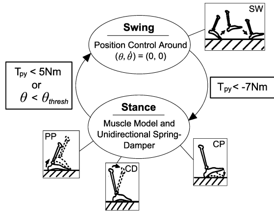
Fig. 2. Finite state machine with state transition thresholds and equivalent ankle-foot biomechanics during each state. Swing is labeled SW, and stance is divided into controlled plantar flexion (CP), controlled dorsiflexion (CD) and powered plantar flexion (PP) as in [5]. State transitions are determined using the prosthetic ankle torque, T_p , as measured from the pyramid strain gauges, and prosthesis ankle angle, \theta .
