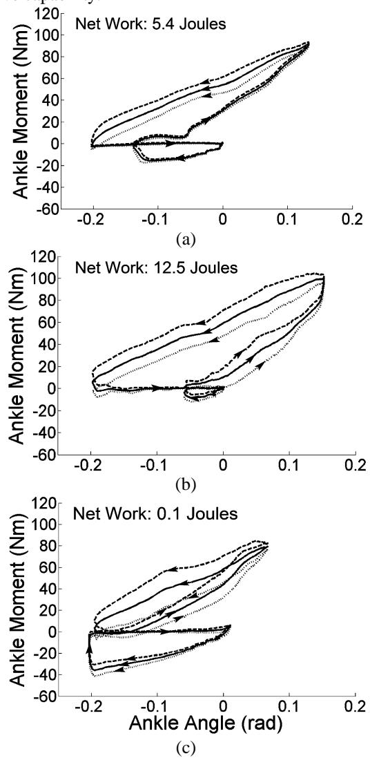
Fig. 9. Measured prosthesis torque-angle trajectories for three different walking conditions: level ground (a), ramp ascent (b), and ramp descent (c). Shown are mean \pm one standard deviation. Arrows indicate forward propagation in time. The average prosthesis net work increases with increasing ground slope. This result is consistent with human ankle data from the literature [35].
