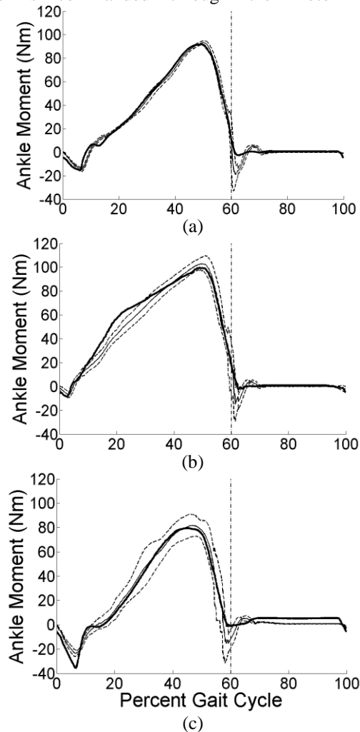
Fig. 4. Prosthesis torque tracking over one complete gait cycle (heel-strike to heel-strike of the same foot) for three walking conditions: level-ground (a), ramp ascent (b), and ramp descent (c). Shown are commanded torque mean \pm standard deviation (thin line), and prosthesis torque, as estimated using the measured SEA torque contribution and angle-based estimate of the parallel spring torque contribution (thick line). The vertical (dash-dot) line indicates the end of the stance phase.
