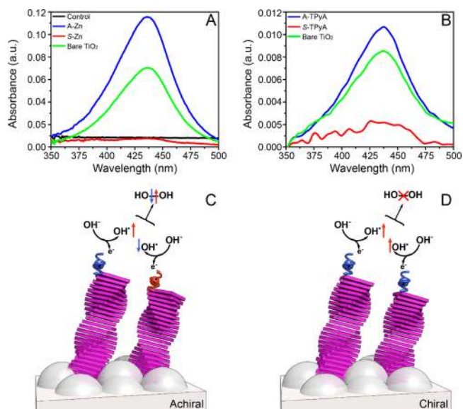
Figure 4. Control of the hydrogen peroxide production. UV–vis absorption spectra from the titration of the used electrolyte (Na 2 SO 4 ) with o -tolidine of TiO 2 and TiO 2 electrodes coated with (A) self-assembled Zn-porphyrins of either achiral (A-Zn) or chiral (S-Zn) and (B) TPyA molecules. The control refers to the titration of unused Na 2 SO 4 with o -tolidine. (C) When the electrons transfer to the anodes is non spin specific the spins of the unpaired electrons on the two OH* are aligned antiparallel, hence the interaction between the two OH* is on a singlet surface that correlates with the production of hydrogen peroxide (H 2 O 2 ). (D) When the electron transfer to the anode is spin specific, the spins of the two electrons are aligned parallel to each other, hence the two OH* interact on a triplet surface that forbids the formation of H 2 O 2 and facilitates the production of oxygen in its ground state.
