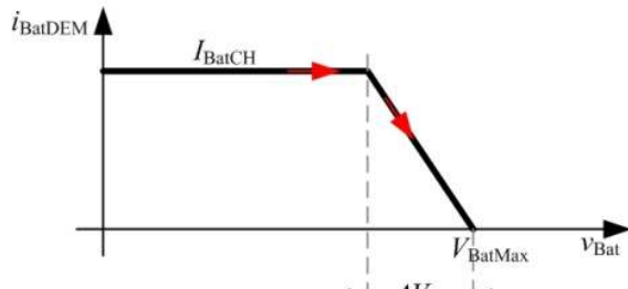
Fig. 6. Battery charging limitation function.
