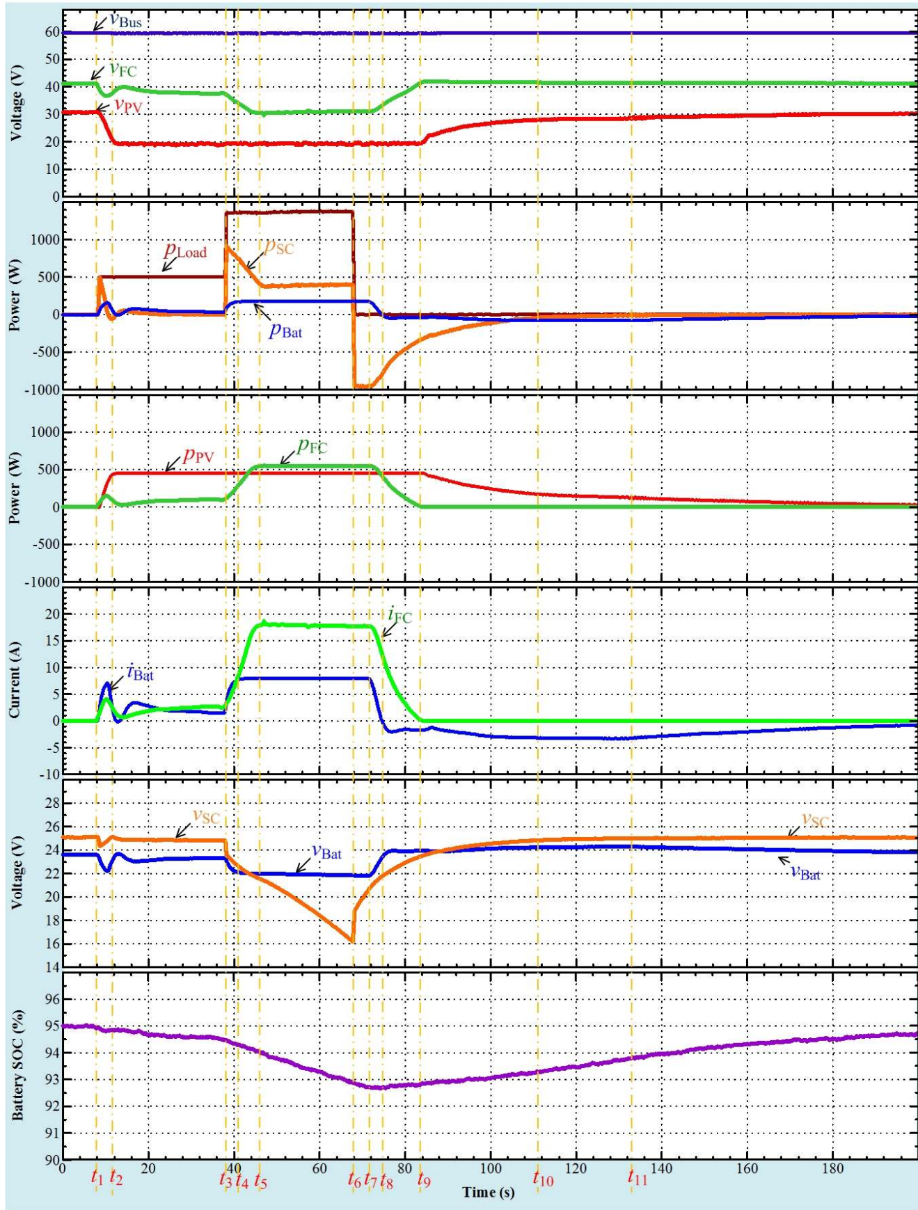
Fig. 9. Experimental results: power plant response during long load cycles.
