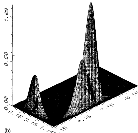
FIG. 9. (a) The absolute square of the product between the |0,0\rangle state and the transition dipole function superimposed on the potential energy surface of the first electronically excited state (dashed lines). (b) Dissociation dynamics in the first electronically excited state of HOD starting with the state of (a). The absolute square of the wave function is shown after 15 fs time evolution.
