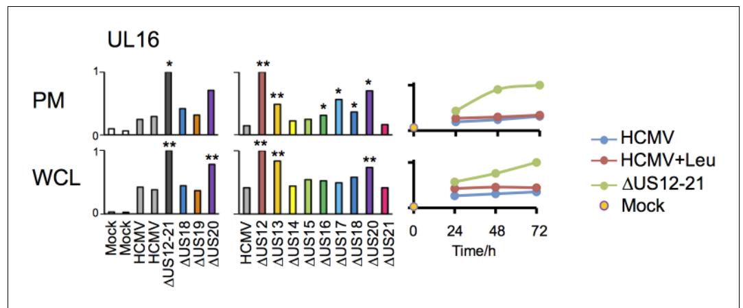
Figure 9. Regulation of UL16 levels by the US12 family. Quantitation of UL16 in proteomic series 1–3 in both PM and WCL. Relative abundance of each protein is expressed relative to the sample with the highest abundance (set to 1). For proteomic series 1 and 2, p values were calculated as described in Figure 4 : * p < 0.05 , ** p < 0.0001 . DOI: 10.7554/eLife.22206.012
