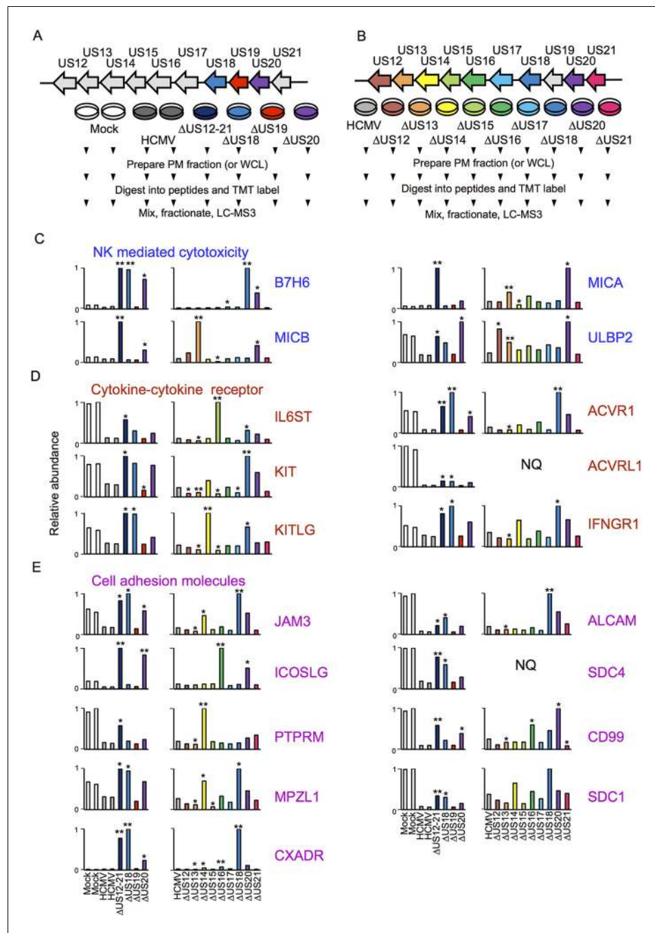
Figure 4. Proteomic analysis of cellular proteins targeted by US12 family members in PM samples. (A-B) Workflows of proteomic series 1 and 2 respectively. (C-E) Quantitation of PM proteins in enriched KEGG pathways identified using DAVID. Relative abundance of each protein is expressed relative to the sample with the highest abundance (set to 1). NQ – not quantified. A number of the US12-21 mutant targets were also regulated by the US18 and US20 mutants (B7-H6, ULBP2, IL6ST, KIT, KITLG, JAM3, ACVR1, ACVRL1, IFNGR1, JAM3, MPZL1, CXADR, ALCAM, SDC4, CD99, SDC1). A subset of these proteins were also regulated by the US14 and/or US16 mutants (KIT, KITLG, ACVR1, IFNGR1, JAM3, MPZL1, CD99, SDC1). We estimated p values for the ratios of each mutant compared to HCMV Merlin using Benjamini-Hochberg corrected Significance B values (Cox and Mann, 2008): * p < 0.05 , ** p < 0.0001 . For proteomic series 1, ratios were calculated as US12 family deletion mutant / average HCMV and for proteomic series 2, US12 family deletion mutant / HCMV. All proteins quantified by 2 or more peptides were included in this calculation. SDC1 was quantified by a single peptide in proteomic series 2. DOI: 10.7554/eLife.22206.007
