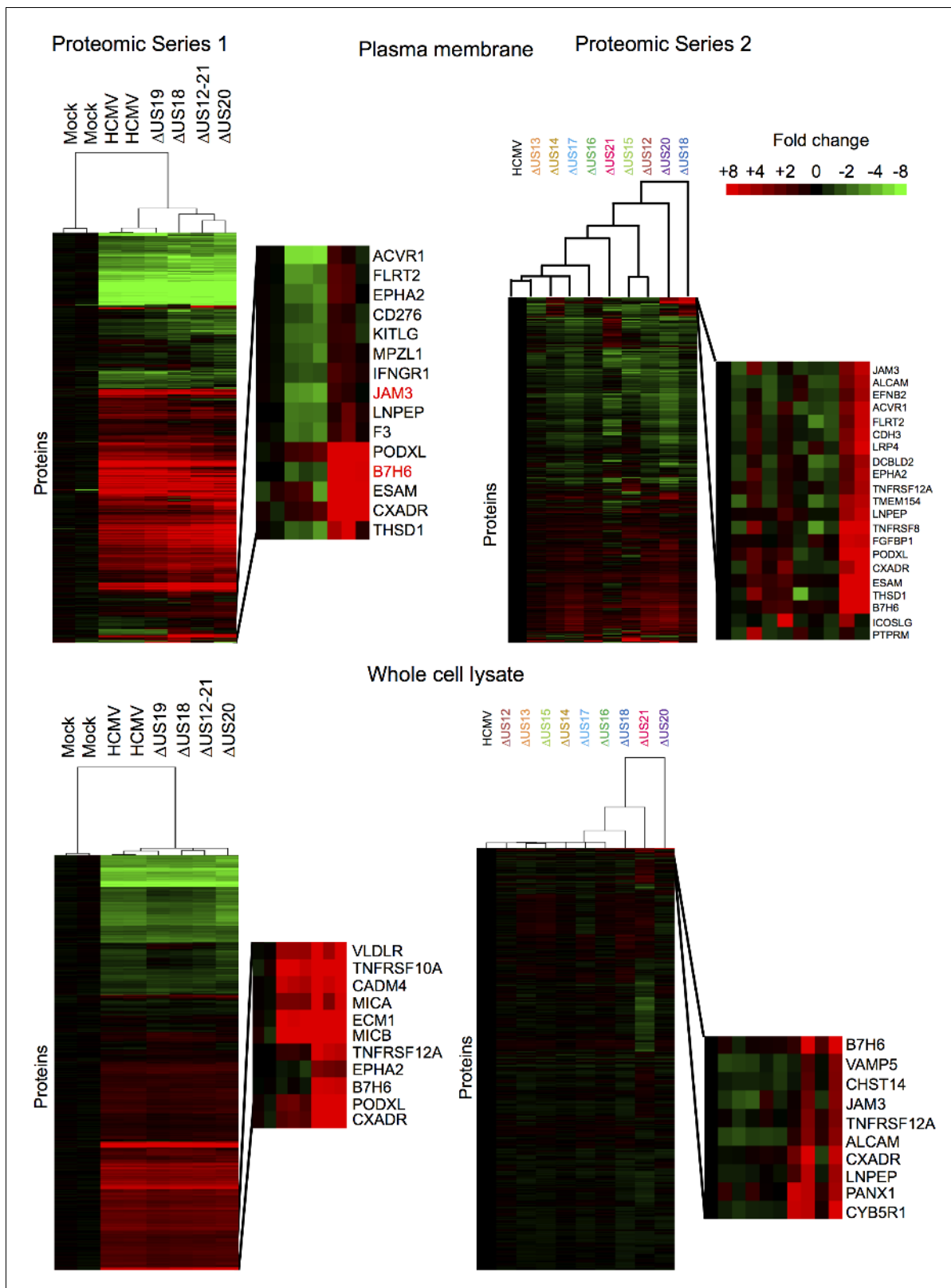
Figure 3. Hierarchical cluster analysis of all proteins quantified in proteomic series 1 and 2. Zoomed regions are shown for clusters of interest.
