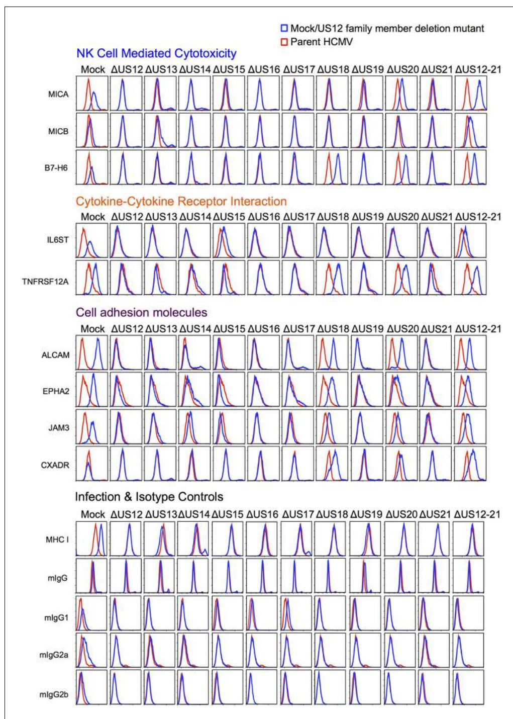
Figure 10. Validation of cell surface proteins regulated by the US12 family. Flow cytometry confirmed proteomic data for proteins representative of each category enriched in the DAVID analysis. Staining in mock/US12 family member deletion mutant infections (blue line) is shown relative to the parental HCMV infection (red line). Flow cytometry was carried out for cell surface expression of MHC I (W6/32) as a control for HCMC infection and isotype antibody staining controls (with directly PE-conjugated IgG1, IgG2a or IgG2b antibodies or for unconjugated antibodies mIgG and an anti-mouse-AF647 conjugated secondary antibody). Infected cells were assessed by the % cells with down-regulated MHC I compared to the mock-infected cells (HCMV 94%, \Delta US12 94%, \Delta US13 94%, \Delta US14 83%, \Delta US15 95%, \Delta US16 97%, \Delta US17 85%, \Delta US18 94%, \Delta US19 96%, \Delta US20 94%, \Delta US21 94%, \Delta US12-21 96%). Results are representative of at least two independent experiments.
