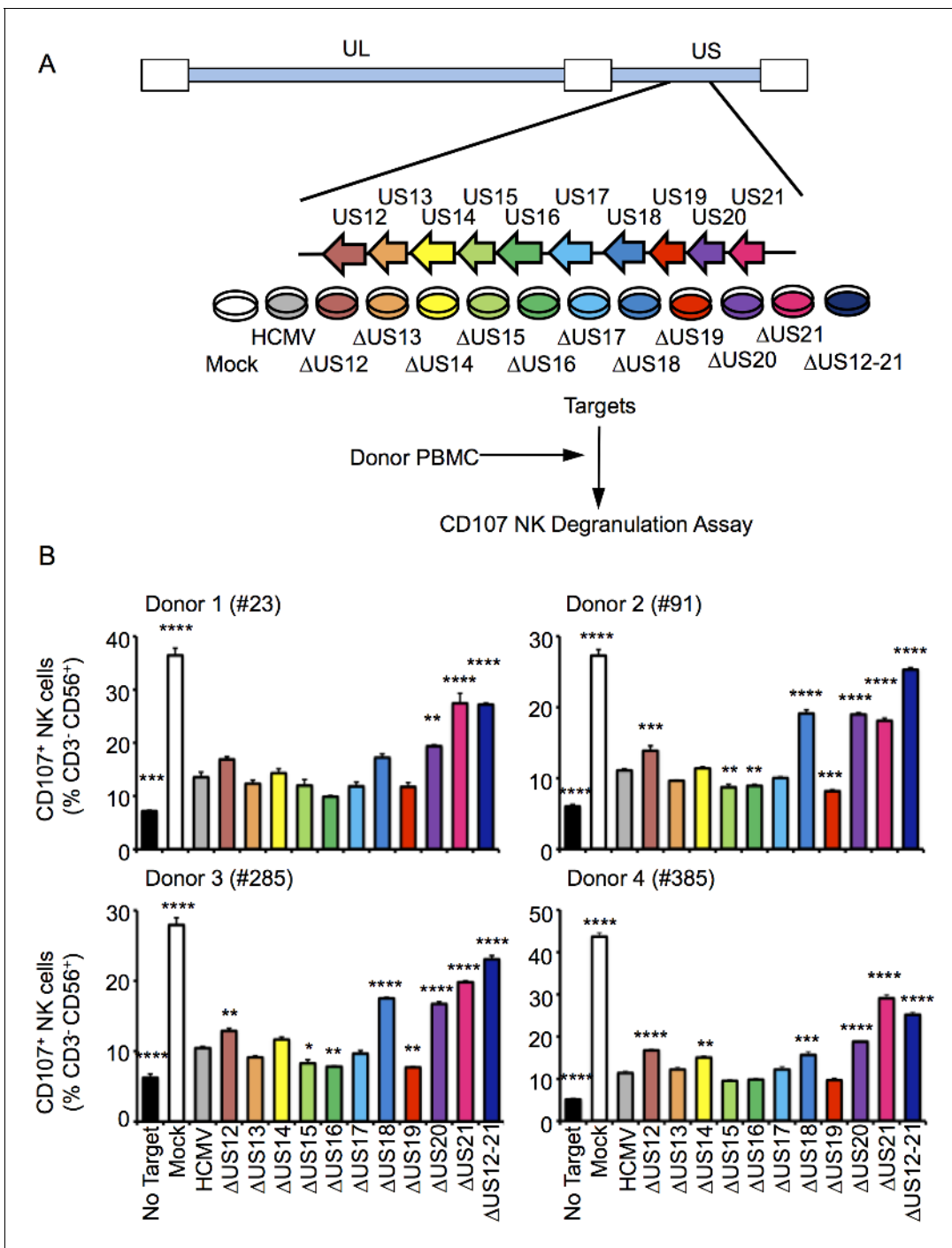
Figure 1. Multiple US12 family proteins regulate NK activation. (A) Fibroblasts (HF-TERTs) were mock infected or infected with the Merlin strain of HCMV or the series of US12 family deletion mutants for 72 hr. Infected cells were incubated with donor PBMC for 5 hr and NK degranulation assessed by % CD107 + cells within the CD3 + , CD56 + population by flow cytometry. (B) CD107 assay results (mean and SD) are shown from four separate donors performed in duplicate or triplicate and analysed by unpaired ordinary one way ANOVA with Dunnett’s test for multiple comparisons against the HCMV control *p<0.05, **p<0.01, ***p<0.005 ****p<0.001). Infected cells were assessed by the % cells with down-regulated MHC I compared to the mock-infected cells (for the experiment using donor #23 and # 385, HCMV 93%, \Delta US12 94%, \Delta US13 98%, \Delta US14 94%, \Delta US15 98%, \Delta US16 99%, \Delta US17 98%, \Delta US18 97%, \Delta US19 99%, \Delta US20 97%, \Delta US21 91%, \Delta US12-21 94%; for the experiment using donor #91 and # 285, HCMV 94%, \Delta US12 94%, \Delta US13 94%, \Delta US14 83%, \Delta US15 95%, \Delta US16 97%, \Delta US17 85%, \Delta US18 94%, \Delta US19 96%, \Delta US20 94%, \Delta US21 94%, \Delta US12-21 96%).
