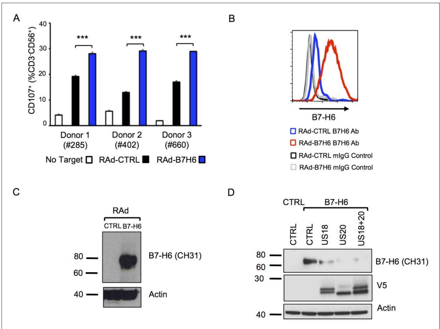
Figure 11. Adenovirus expressed B7-H6 regulates NK cell activation and B7-H6 levels are regulated by ectopically-expressed US18 and US20. (A) HF-CARs were infected with control (RAAd-CTRL) or B7-H6-expressing (RAAd-B7-H6) adenovirus vectors (MOI 5). Cells were harvested 48 h p.i. and used as targets in a CD107 degranulation assay with buffy-coat derived PBMC from 3 separate donors in duplicate or triplicate. Results (shown as mean and SD) were analyzed by unpaired two-tailed Student's T-test. *** p < 0.001 , **** p < 0.0001 . (B and C) HF-CARs were infected with control (RAAd-CTRL) or B7-H6-expressing (RAAd-B7-H6) adenovirus vectors (MOI 5). Cells were harvested 48 h p.i. and B7-H6 cell surface expression analyzed by flow cytometry (B) or western blot (C). Results are representative of at least 2 independent experiments. (D) HF-CARs were infected with adenovirus control (CTRL), US18-expressing adenovirus, US20-expressing adenovirus or a combination of both US18 and US20 (MOI 5 each, made up to a total MOI of 10 with RAAd-CTRL). After 24 hr incubation, HF-CARs were infected with adenovirus control (CTRL) or B7-H6-expressing adenovirus (B7-H6) at MOI 5 as indicated before incubation for a further 48 hr. Whole cell lysates were prepared and analysed by immunoblotting with the antibodies indicated. Results are representative of two independent experiments.
