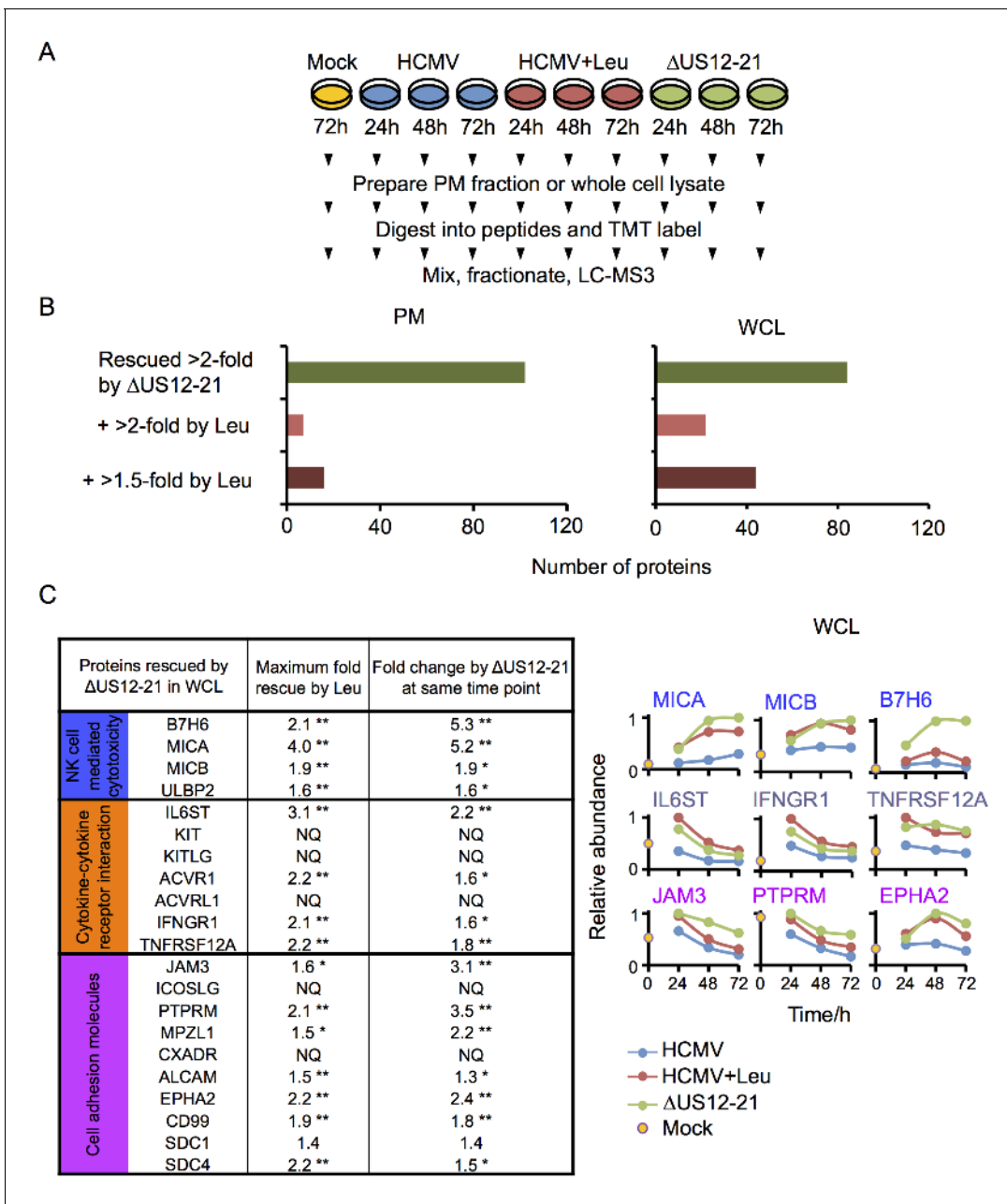
Figure 8. Multiple US12 gene family targets are degraded via the lysosomal pathway. (A) Workflow of Proteomic Series 3. (B) Number of proteins targeted by the US12-21 block and additionally rescued >2 fold in the dataset by the \Delta US12-21 deletion mutant or rescued >2 fold or >1.5 fold by leupeptin treatment for both WCL and PM. C. Comparable degree of rescue of US12-21 target proteins by US12-21 deletion and leupeptin treatment. Quantitation of a subset of these proteins is shown relative to the maximum abundance (set to 1). p-values were calculated as described in Figure 4 , for the ratios of leupeptin treatment or US12-21 deletion virus infection at each time point compared to the matched wild-type Merlin-infected control. *p<0.05, **p<0.0001. SDC1 was only quantified by one peptide.
