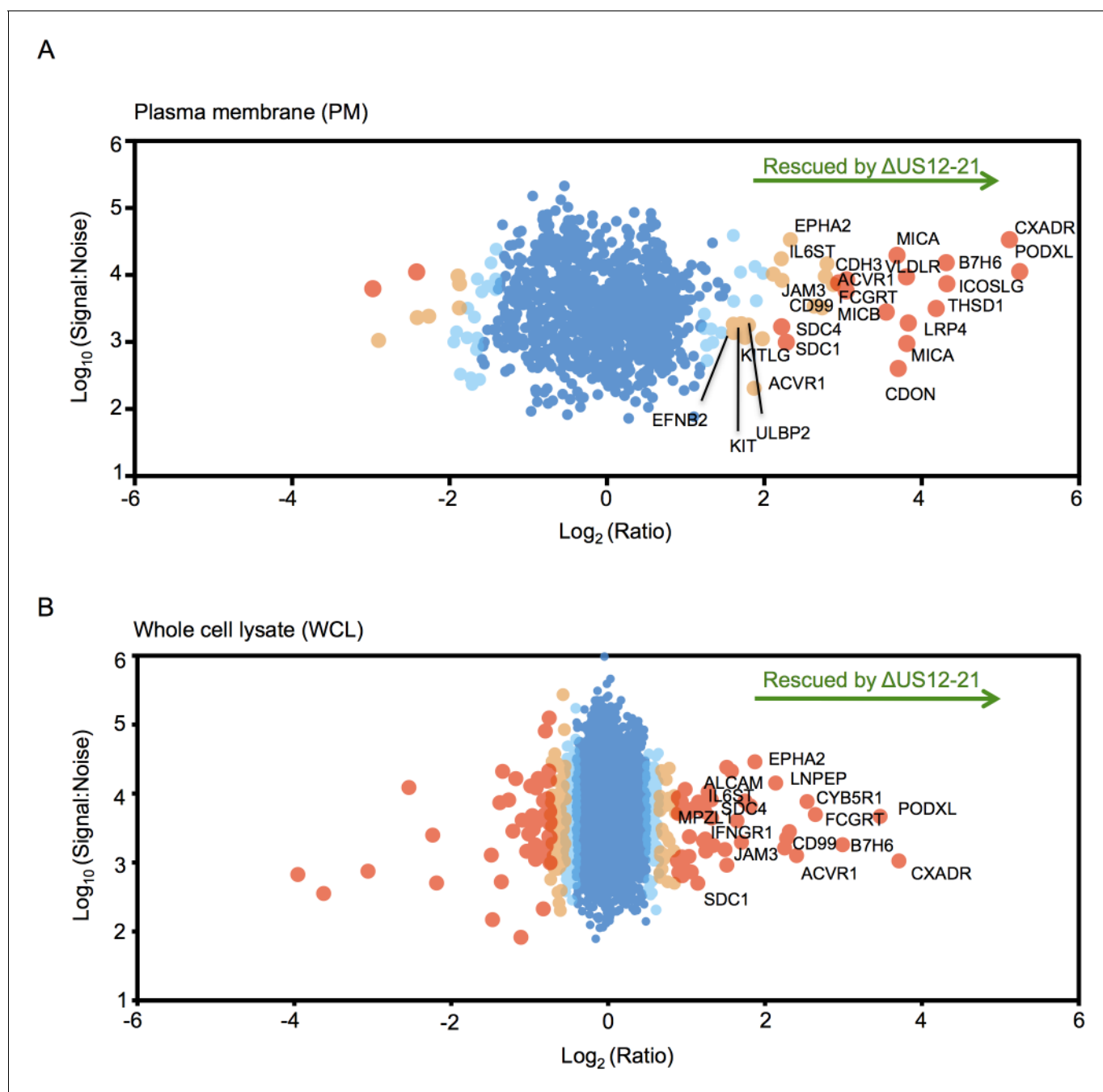
Figure 2. The US12 family targets numerous plasma membrane proteins. Cells infected with HCMV (Merlin) or HCMV \Delta US12-21 mutant were processed to give PM or WCL fractions and analyzed by TMT mass spectrometry. Scatter plot of proteins identified in the PM (panel A) or WCL fractions (panel B) respectively and quantified by 2 or more unique peptides. Fold change ( \Delta US12-21-infected fibroblasts/HCMV-infected cells) is shown as the log 2 ratio on the x-axis and the signal:noise on the y-axis as log 10 . Proteins unaltered by the US21-21 deletion locate at the center of the plots (0 log 2 /1 fold-change), whereas proteins to the left or right of center represent proteins down- or up-regulated by the US12-21 deletion respectively. Significance B was used to estimate p values (Cox et al., 2009). The 2 different alleles of MICA present in HFs were detected by this analysis.
