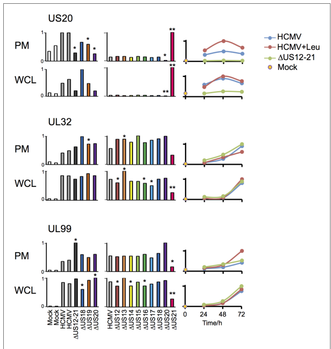
Figure 7. Altered expression of US20, UL32 and UL99 levels in the US21 deletion mutant-infected fibroblasts. Quantitation of US20, UL32 and UL99 in proteomic series 1–3 in both PM and WCL. Abundance of each protein is expressed relative to the sample with the highest abundance (set to 1). For proteomic series 1 and 2, p values were calculated as described in Figure 4 : * p < 0.05 , ** p < 0.0001 . US20 was only quantified by one peptide in proteomic series 1, WCL experiment.
