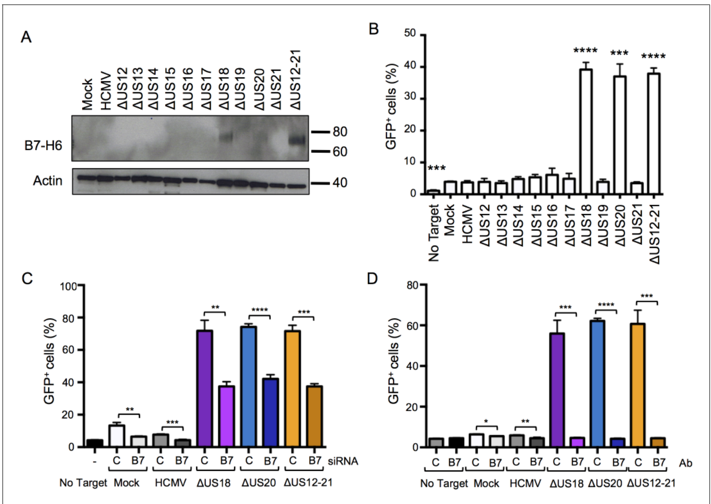
Figure 12. Differences in B7-H6 levels on HCMV US12 family deletion mutant-infected cells regulate NKp30-mediated responses. (A) Whole cell lysates were prepared from mock, HCMV or the series of US12 family deletion mutant infected fibroblasts and analyzed by immunoblotting with antibodies specific for B7-H6 (CH31) or actin. Results are representative of two independent experiments. (B) An NKp30-responsive 2B4 reporter cell line containing a NFAT-GFP reporter construct (CT299) was incubated for 24 hr with mock, HCMV or the series of US12 family deletion mutant infected fibroblasts in triplicate. Fixed cells were then analyzed for GFP fluorescence by flow cytometry compared to cells incubated with no target fibroblasts. Results are expressed as the % GFP positive reporter cells (mean and SD) and were analyzed by unpaired two-tailed Student's T-test. Results are representative of two independent experiments. (C) HF-TERTs were transfected with control (C) or B7-H6 (B7) siRNAs for 24 hr prior to infection with the parent HCMV, \Delta US18, \Delta US20 or \Delta US12-21 mutants for 72 hr. Cells were then incubated for 24 hr with CT299 NKp30 reporter cells in triplicate and GFP + cells determined by flow cytometry, and analysed by unpaired two-tailed Student's t-test. Results (mean and SD) are representative of two independent experiments. (D) HF-TERTs infected with HCMV, \Delta US18, \Delta US20 or \Delta US12-21 mutants were incubated for 24 hr with CT299 NKp30 reporter cells, in the presence isotype control (C) or B7-H6 blocking antibodies (B7) in triplicate, GFP + cells determined by flow cytometry and analyzed by unpaired two-tailed Student's t-test. Results (mean and SD) are representative of two independent experiments.
