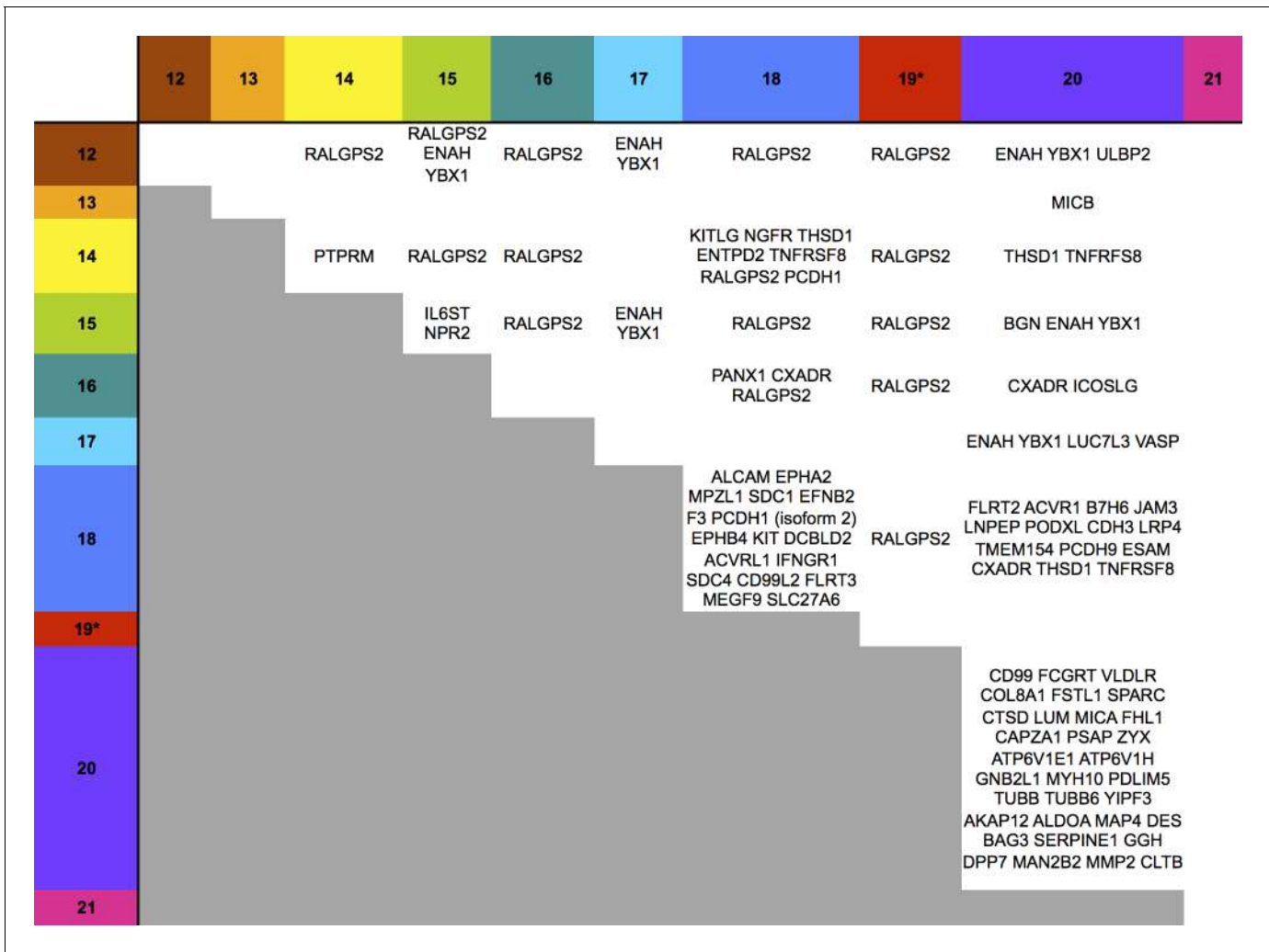
Figure 6. Co-regulation of multiple cell surface proteins by >1 US12 family gene. Proteins that were rescued by deletion of each US12 family member in the PM fraction of proteomic Series 2 (i.e. not including US19) were analyzed to determine which were additionally targeted by one or more US12 family members. Proteins were plotted in a matrix with unique protein targets on the lower diagonal of the plot (US12 family member compared with itself) and common protein targets in intersections with other US12 members. To identify the highest confidence targets of the US12-21 family for the purposes of this analysis and to generate a shortlist of US12-21 family PM ‘hits’, we employed the following strategy: we included proteins (a) exhibiting at least 3-fold rescue upon deletion of a given US12 family member, quantified by at least two peptides and annotated by GO to indicate a PM location. (b) validated by a corresponding >2 fold change in at least one of (i) deletion of the US12-21 block (proteomic series 1 or 3), (ii) the biological repeat of US18 or US20 in proteomic series 1, (iii) the corresponding gene deletion in WCL proteomic series 2. This strategy identified all proteins shown in Figure 3 . *US19 data was used from proteomic series 1.
