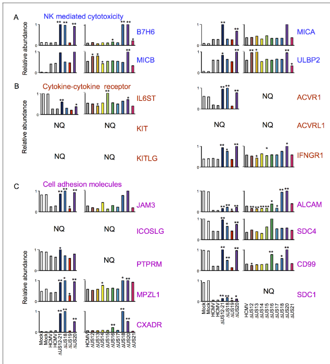
Figure 5. Individual US12-family proteins target key natural killer cell ligands, cell adhesion molecules and cytokines and their receptors in WCL samples. (A–C) Quantitation of key US12 family targets in WCL samples (proteomic series 1 and 2 - comparative analysis of these proteins from PM samples is shown in Figure 3 ). We generally observed similar results for proteins quantified in both PM and WCL samples. Relative abundance of each protein is expressed relative to the sample with the highest abundance (set to 1). NQ – not quantified. P values were calculated as described in Figure 4 : * p < 0.05 , ** p < 0.0001 . MICB was only quantified by 1 peptide in proteomic series 1, and MICA, JAM3 and SDC4 by one peptide in proteomic series 2.
