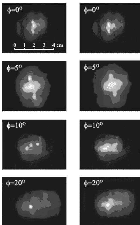
Fig. 3. Filamentation pattern. Left, typical single shot; right, averaged over 1000 shots.
