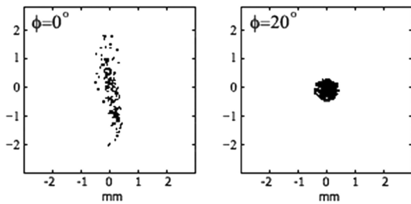
Fig. 4. Location of the central filament in 320 shots.
