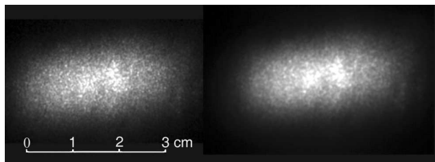
Fig. 1. Input beam spatial profile. Left, typical single shot; right, averaged over 100 shots.
