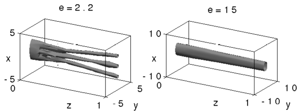
Fig. 5. Solution of Eq. (1) with \varepsilon_{\text{sat}} = 0.005 and input power of 15P_{\text{cr}} .
