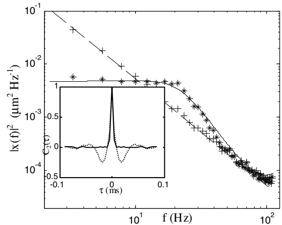
FIG. 3. Power spectra of the x fluctuations of a trapped 50 nm particle (*) and of the corresponding pseudo-free trajectory (+). The trapped spectrum is fit by Eq. (3), with \delta t = 4.5 ms, \alpha = 0.3 , and \Delta = 1.3 . The value of D is fixed at the value extracted from the pseudo-free power spectrum ( 8.7 \mu\text{m}^2 \text{s}^{-1} ). The pseudo-free spectrum is fit by |x(f)|^2 = D/(\pi f)^2 . Inset: normalized two-point correlation functions of the displacements between successive frames along the x axis, C_2(\tau) \propto \langle \delta x(t) \delta x(t + \tau) \rangle . The correlation function of the measured trajectory (dashed line) shows ringing due to the feedback delay, while that of the pseudo-free trajectory (solid line) shows \delta -correlated steps.
