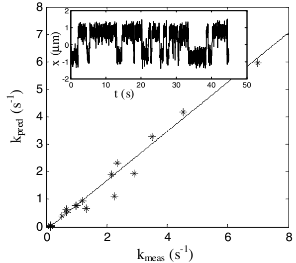
FIG. 5. Comparison of experimental and theoretical hopping rates for a 200 nm particle in a double potential well. Eight trajectories were acquired (10000 data points each), leading to 16 experimental rates (left \rightarrow right and right \rightarrow left for each trajectory). The trend line has a slope of 0.89 (ideal = 1), which is reasonable given the uncertainties in the size of the particle. Inset: the representative trajectory of a single particle.
