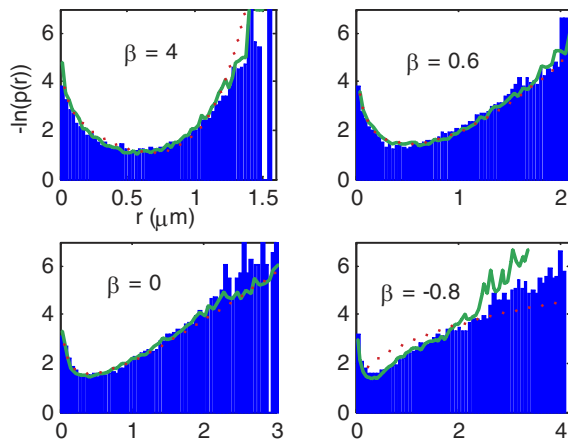
FIG. 4 (color online). Radial probability distributions [plotted as -\ln p(r) ] for a 200 nm particle in a power-law potential. Blue bars: measured distribution; red dots: Eq. (5); green line: numerical simulation.
