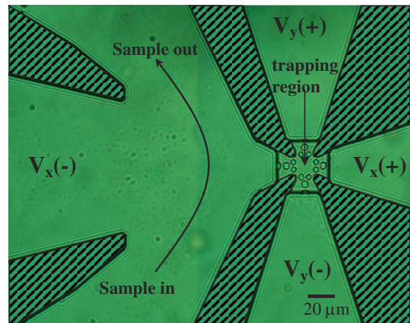
FIG. 1 (color online). Microfluidic cell, formed from an oxidized polydimethylsiloxane (PDMS) stamp and a glass cover slip. The trapping region ( \sim 20 \mu\text{m} across and 880 \text{ nm} deep) allows free in-plane diffusion of submicron particles, while confining the particles to the focal plane of the microscope. Small circles surrounding the trapping region are support posts to keep the PDMS from collapsing onto the glass. Microfluidic channels ( \sim 20 \mu\text{m} deep, \sim 700 \mu\text{m} wide, and \sim 7 \text{ mm} long) radiate outward from the trapping region and terminate in macroscopic copper electrodes. The channel on the left splits into three to allow for rapid sample delivery. Regions of PDMS in contact with the glass have been crosshatched for clarity.
