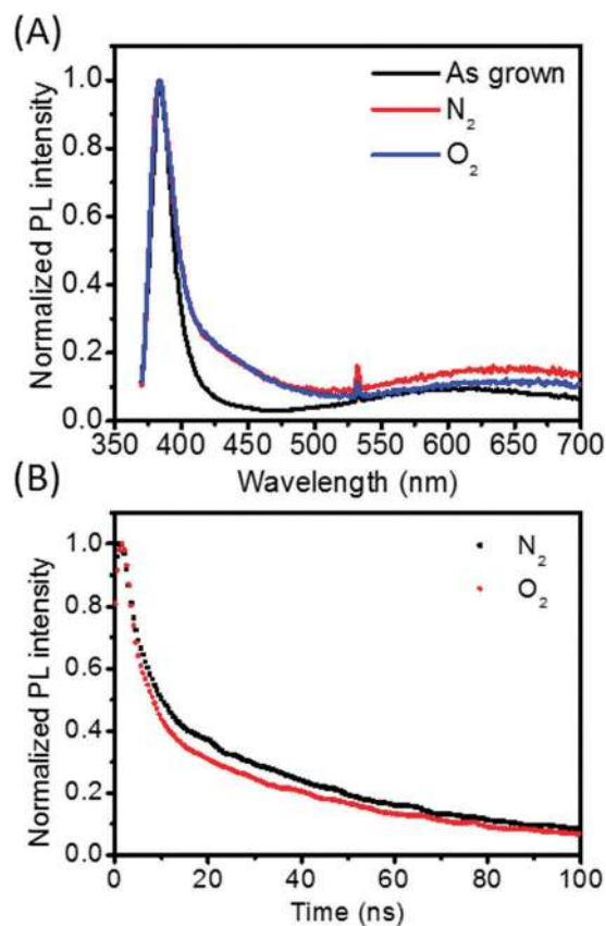
Fig. 7 (A) Integrated photoluminescence spectra of ZnO/PEDOT:PSS annealed in different atmospheres and (B) photoluminescence decay measured at an emission wavelength of 430 nm.
