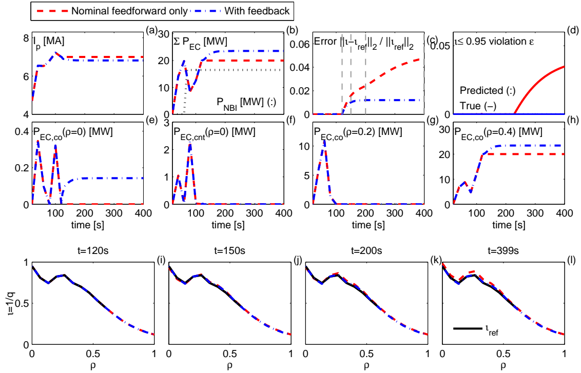
Figure 9. Tracking of reference \nu -profile in flat-top phase. Case with feedforward only (---) is shown together with feedback case (-.-). Top panels show time evolution of actuator commands of plasma current I_p (a), four EC-beams (e-h) and corresponding total EC-power (b) error norm (c) and soft constraint violation (d). Bottom panels reveal \nu -profiles at time steps also indicated by gray dotted lines in top panels (120, 150, 200 and 399 s). Reference \nu -profile is also shown for comparison (-). Feedback controller reduces the tracking error (c) and avoids the soft constraint violation (d) by adjusting the actuators (a,e,h).
