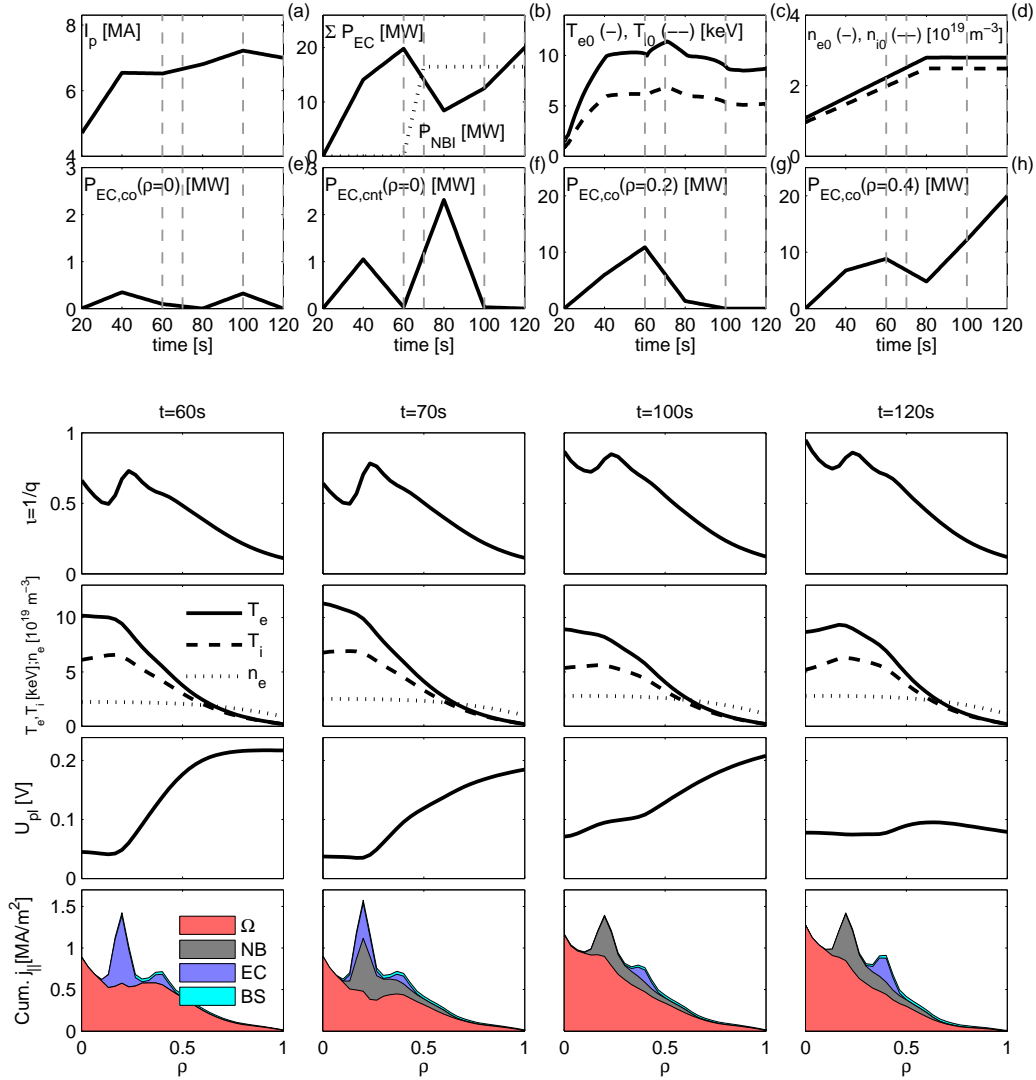
Figure 7. Optimized nominal trajectories for achieving stationary \nu -profile at the beginning of the flat-top phase in L-mode, while satisfying actuator and plasma physics constraints. Top panels show the time evolution of optimal actuator commands of the plasma current I_p (a), four EC-beams (e-h) and corresponding total EC-power (b), central temperatures (c) and central densities (d). The prescribed evolution of NBI-power is also shown in (b). Bottom panels show the profiles \nu, T_{e,i}, n_e, U_{pl} and components of j_{||} at 60, 70, 100 and 120 s. Note I_p(120\text{ s}) = 7\text{ MA} , that is the maximum achievable plasma current in our simulations for achieving a stationary \nu -profile within the given constraints in L-mode.
