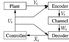
Fig. 1. System with communication channel.
